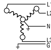
3 Phase Wye 4 Wire + Ground
