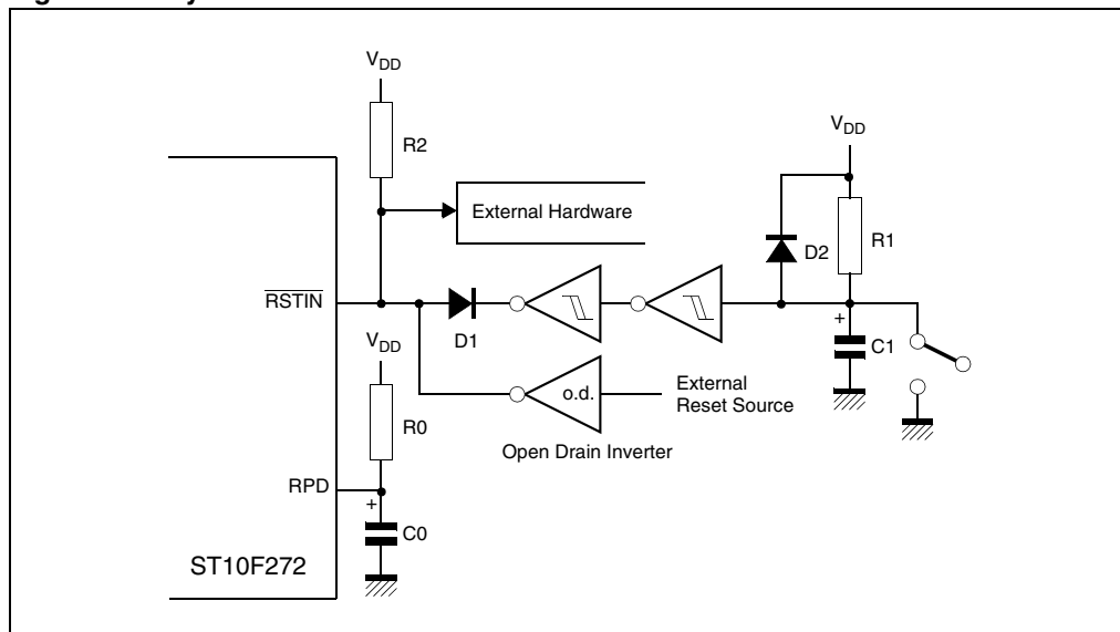
Figure 32. Internal (simplified) reset circuitry
