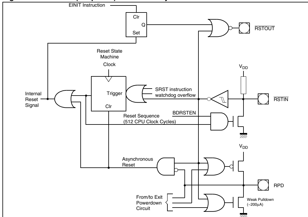
Figure 32. Internal (simplified) reset circuitry
