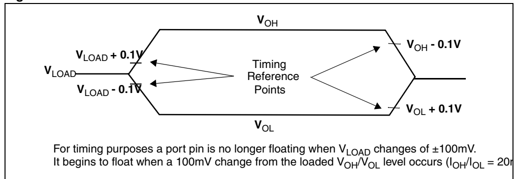
Figure 47. Float waveforms
