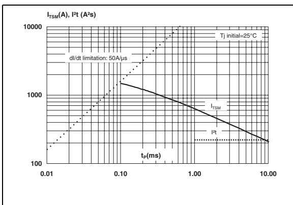
Figure 7. Non repetitive surge peak on-state current (sinusoidal pulse width t_p < 10 \text{ ms} ) and value of I^2t
