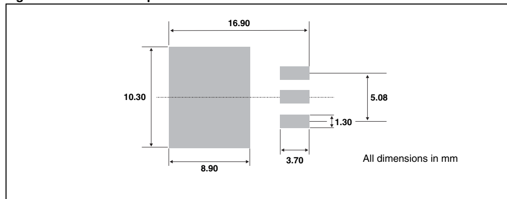
Figure 14. D 2 PAK Footprint
