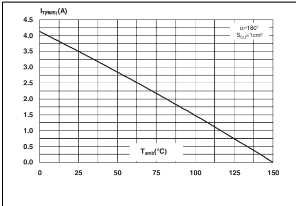
Figure 3. RMS on-state current vs ambient temperature (epoxy printed circuit board FR4 \epsilon_{CU} = 35 \mu\text{m} )
