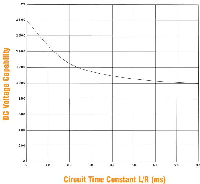
DC VOLTAGE CAPACITY VS. TIME CONSTANT
