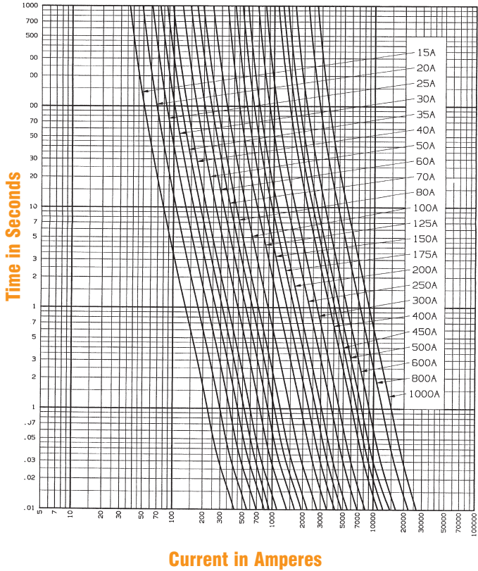
Melting Time – Current Data, 1500V Fuses
