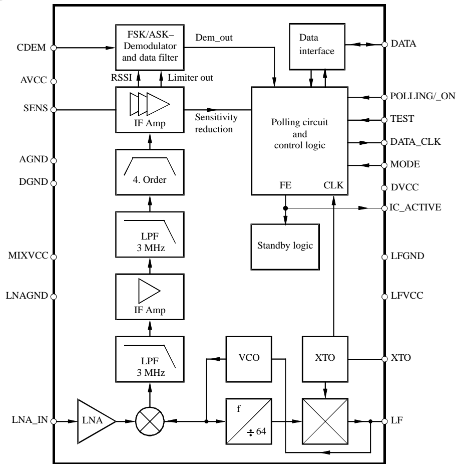
Figure 3. Block diagram
