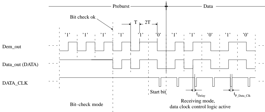
Figure 22. Timing diagram of the data clock
