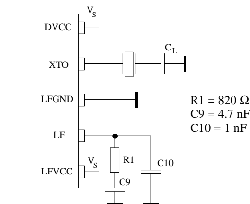
Figure 4. PLL peripherals
