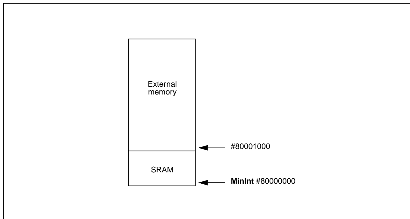
Figure 8.1 SRAM mapping
