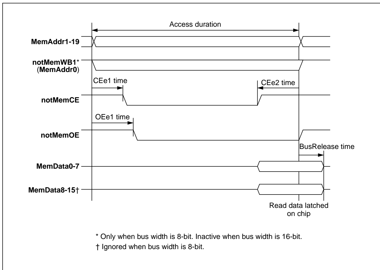
Figure 9.2 Configuration parameters for a read access
