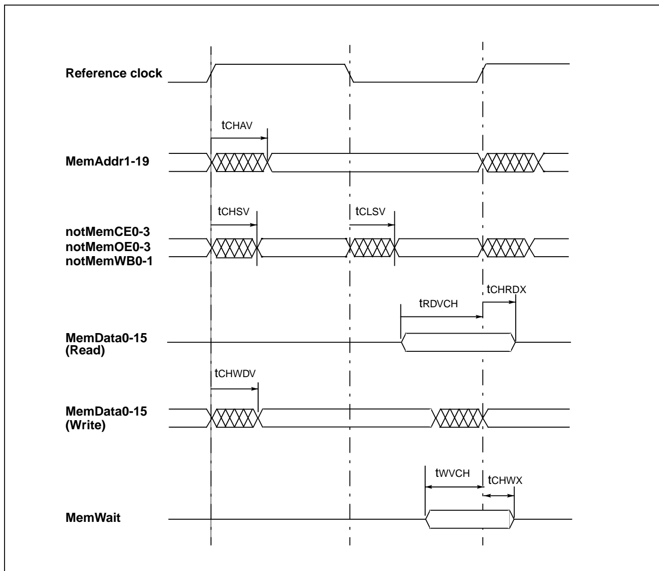
Figure 19.1 EMI timings
