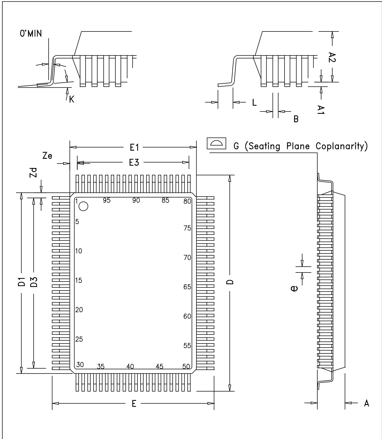
Figure 21.2 100 pin PQFP package dimensions
