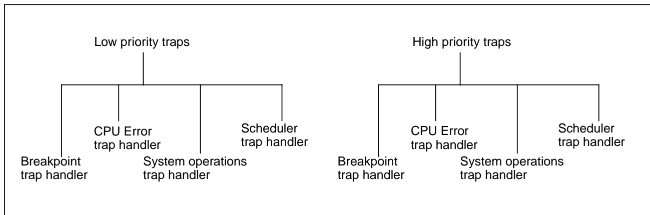
Figure 4.4 Trap arrangement
