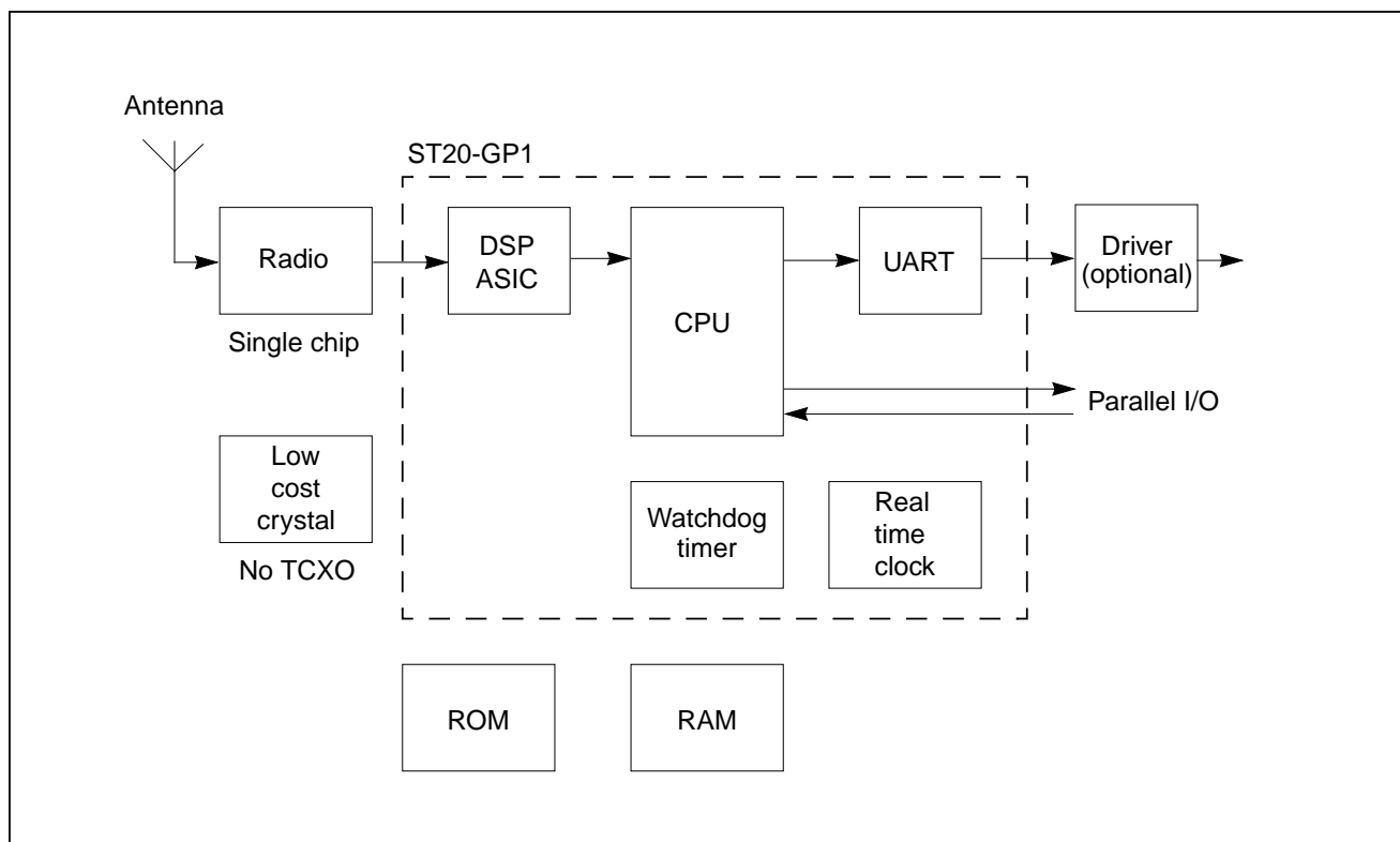
Figure 1.1 GPS system
