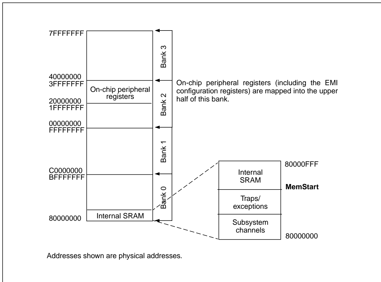
Figure 9.1 Memory allocation
