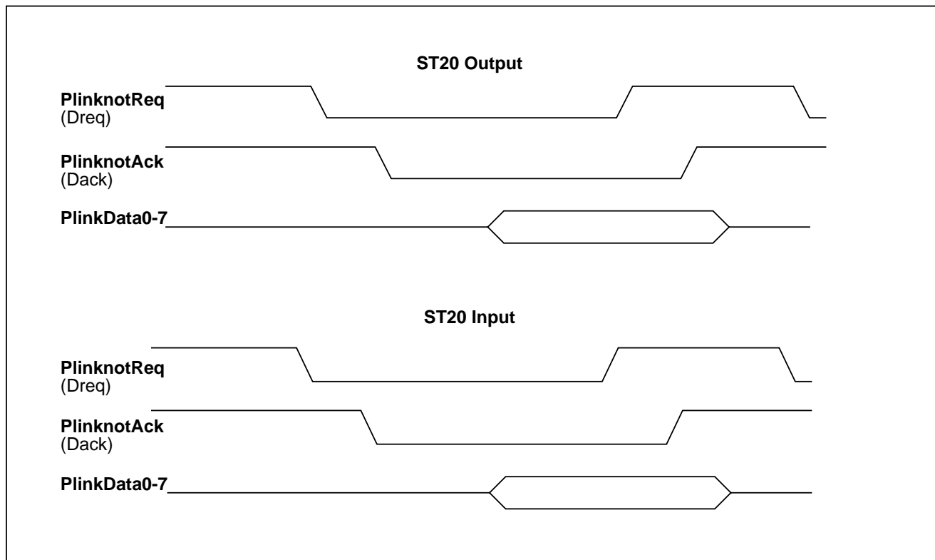
Figure 15.1 Dreq/Dack protocol
