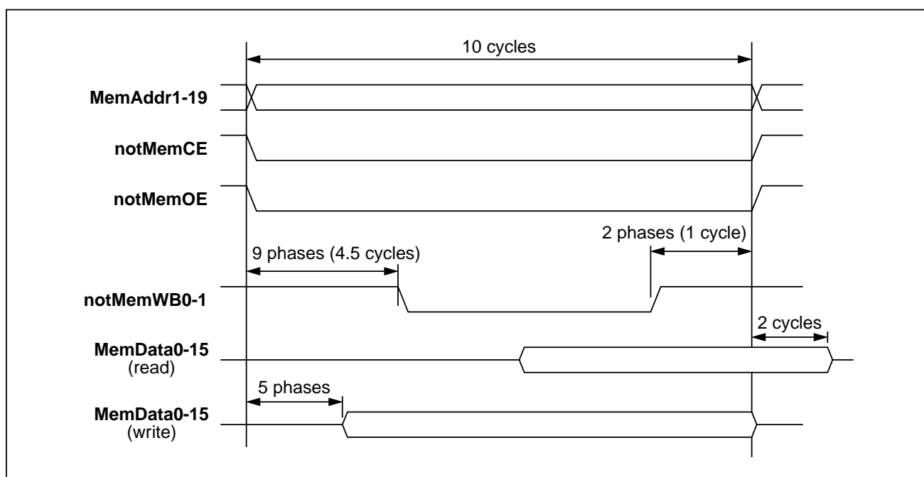
Figure 9.7 Default configuration
