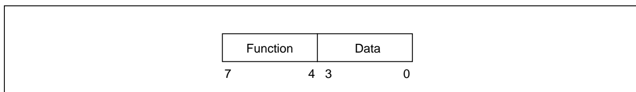
Figure 6.1 Instruction format
