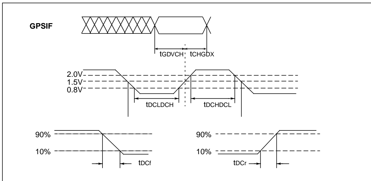
Figure 19.5 ClockIn timings
