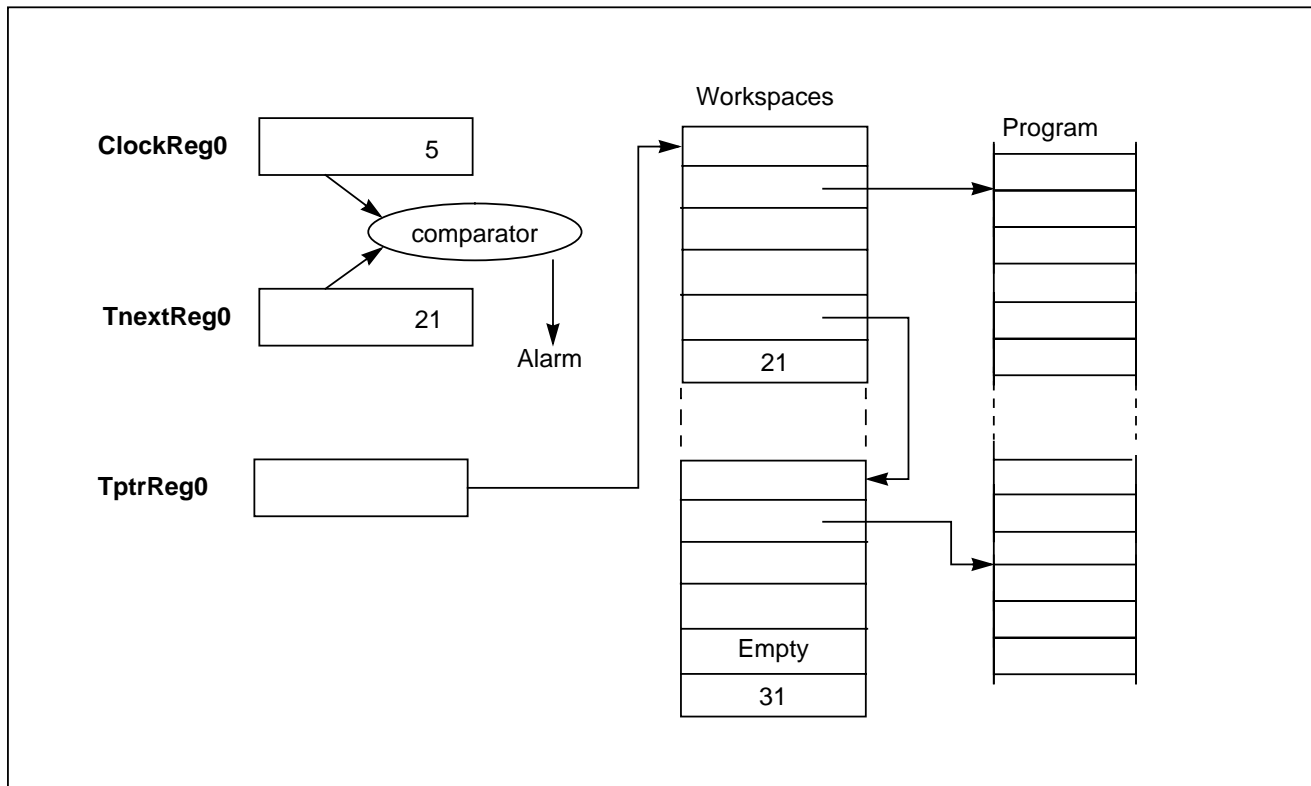
Figure 4.3 Timer registers
