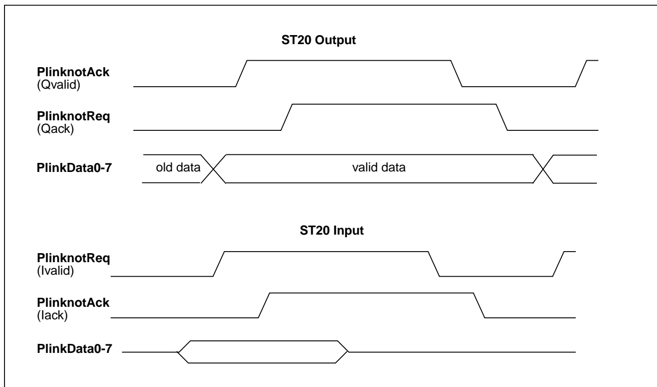
Figure 15.2 Valid/Ack protocol
