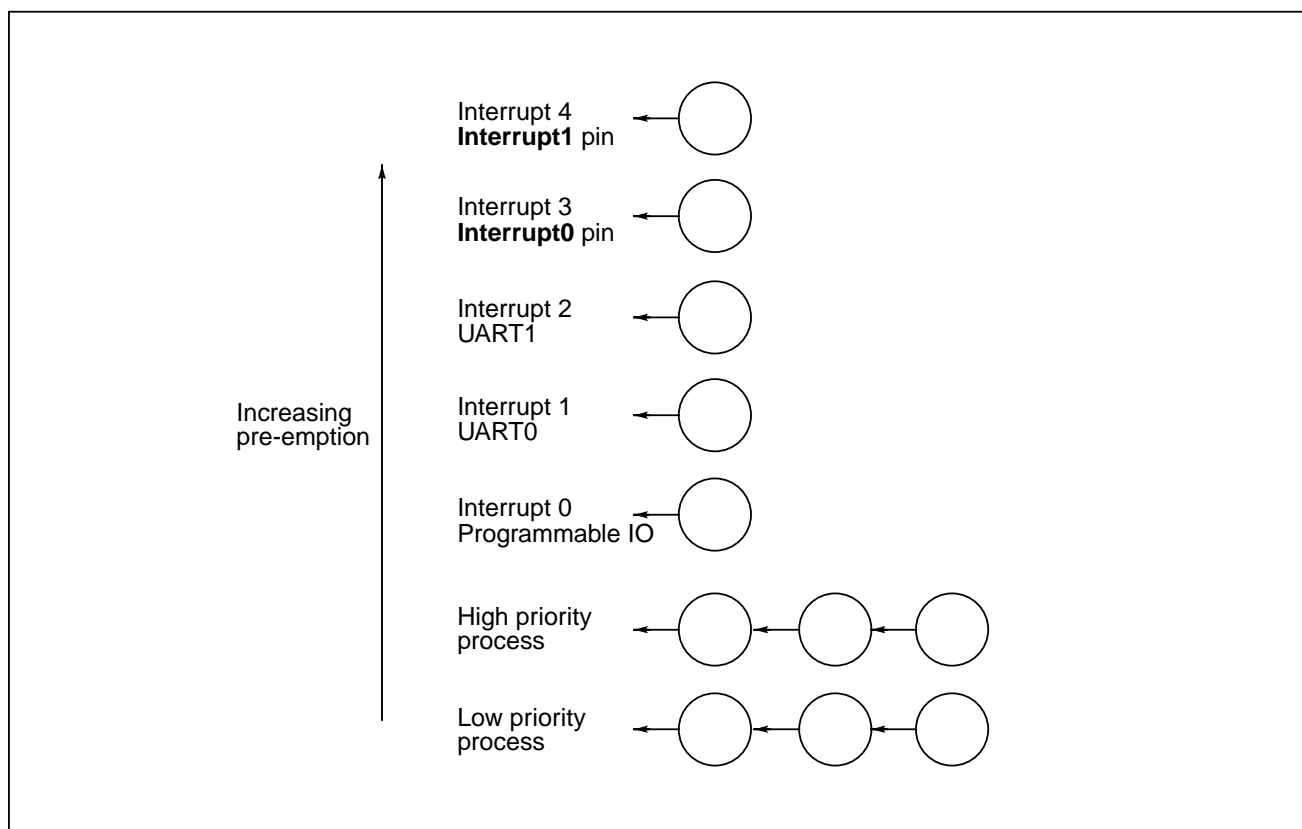
Figure 5.1 Interrupt priority
