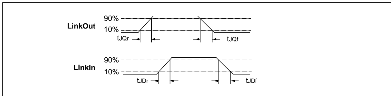
Figure 19.2 Link timings
