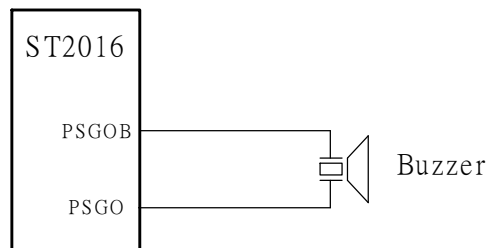
FIGURE 13-15: PSG application circuit
