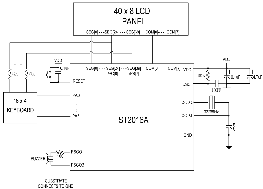
FIGURE 18-32: APPLICATION CIRCUIT WITH LCD KEYBOARD AWAKING PULSE
