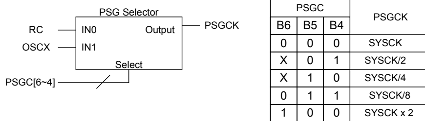
FIGURE 14-17: Clock Source for DAC
