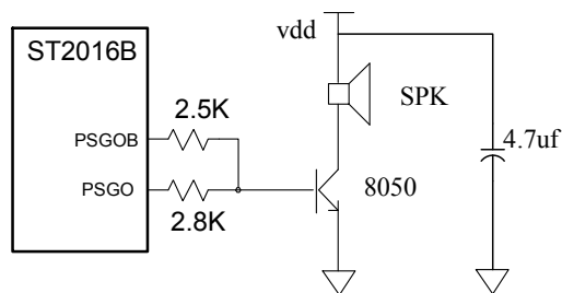
FIGURE 14-21: Two-Pin Two Ended mode Application Circuit
