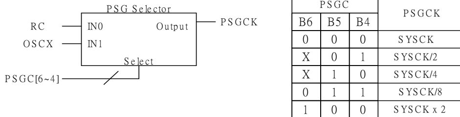
FIGURE 13-10: Clock Source for PSG
