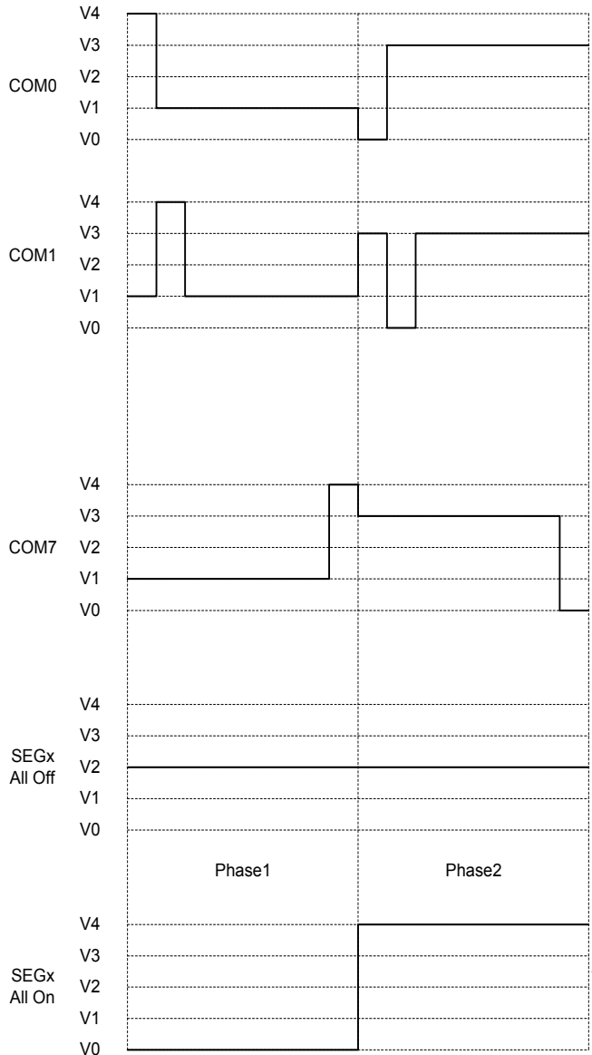
1/8 duty , 1/4 bias LCD signal
