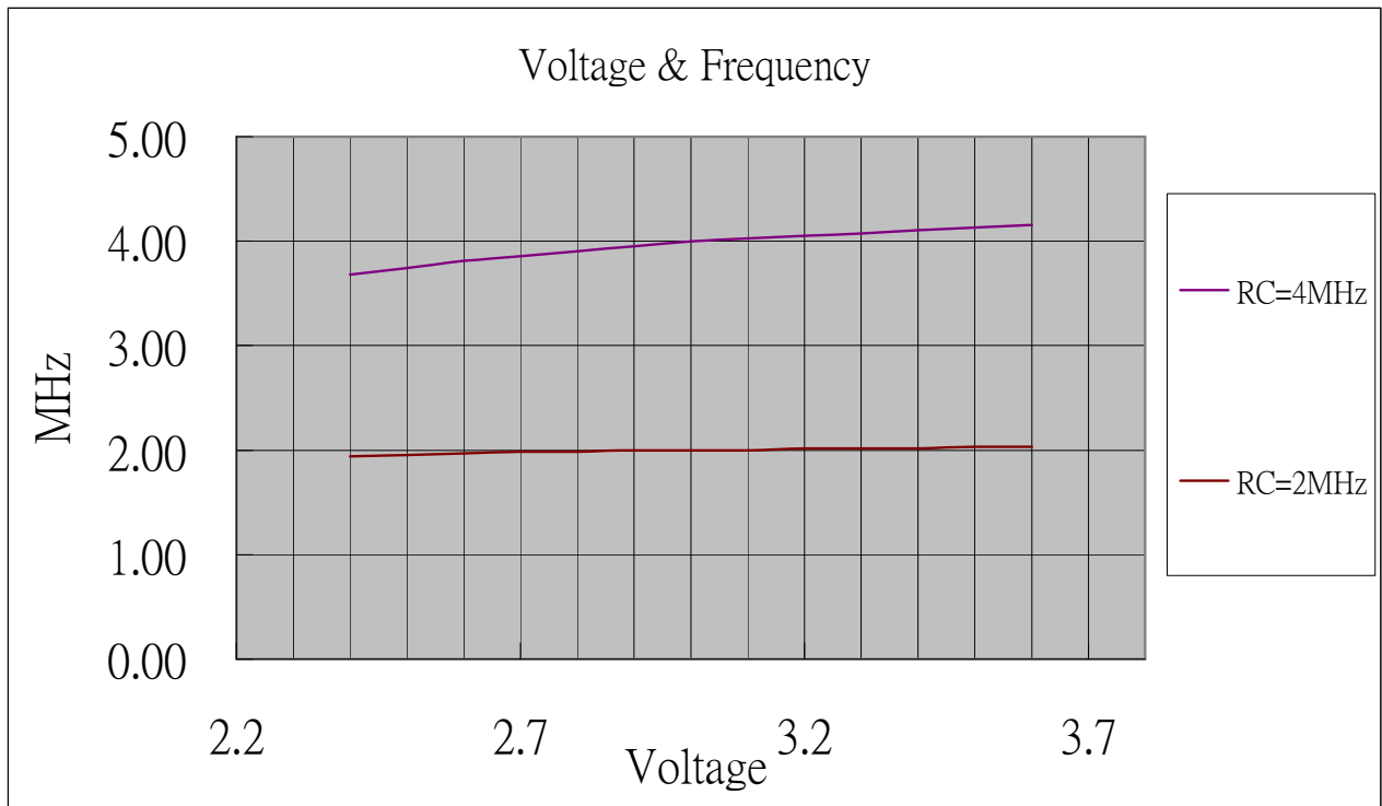
FIGURE 17-29: Relation between operation voltage & frequency
