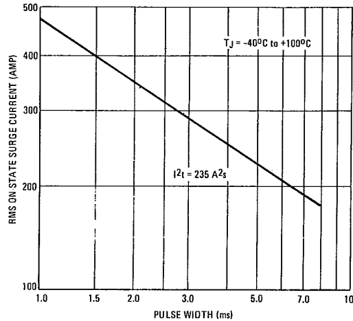
FIGURE 4 - SUB-CYCLE SURGES
