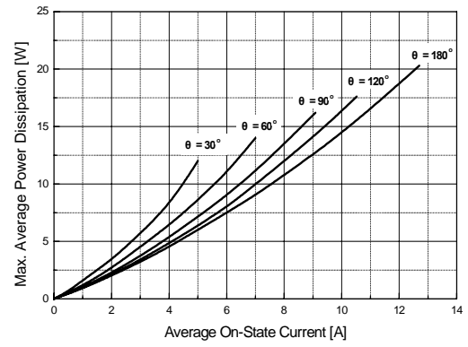
Fig 8. Power Dissipation
