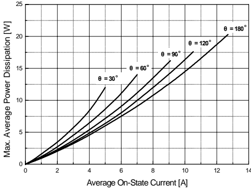
Fig 8. Power Dissipation
