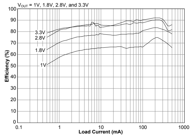
Efficiency vs. I_{OUT} ( T_A = 85^\circ C )
