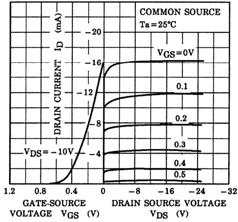
STATIC CHARACTERISTICS
