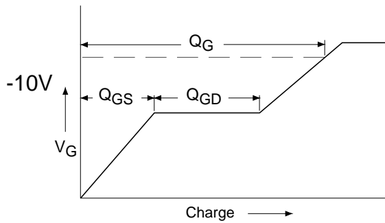
Fig 9a. Basic Gate Charge Waveform
