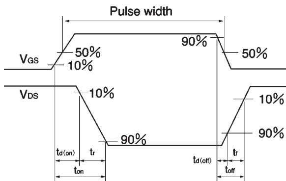
Fig.17 Switching time waveforms
