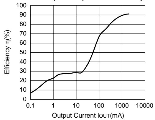
R1224N502H (V IN =12V) CDRH127-10μH
