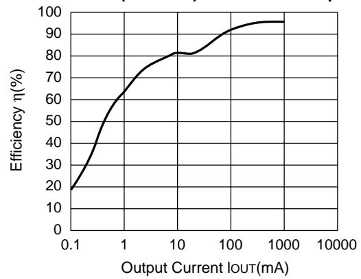
R1224N502L (V IN =6.5V) CDRH127-27μH
