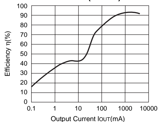
R1224N502G ( V_{IN}=10V )
