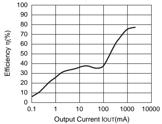
R1224N182H (V IN =12V) CDRH127-10μH
