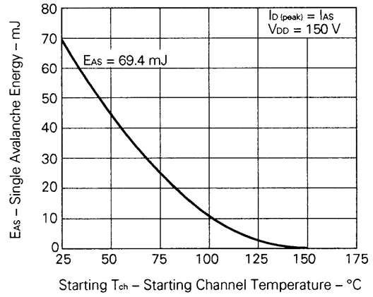
SINGLE AVALANCHE ENERGY vs. STARTING CHANNEL TEMPERATURE
