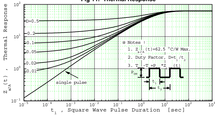
Fig 11. Thermal Response
