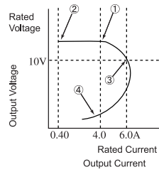
Fig1. Output Voltage/Current
