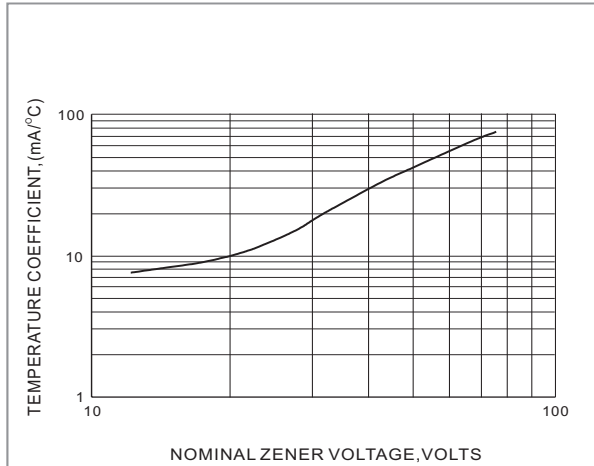
Fig.2 TEMPERATURE COEFFICENTS
