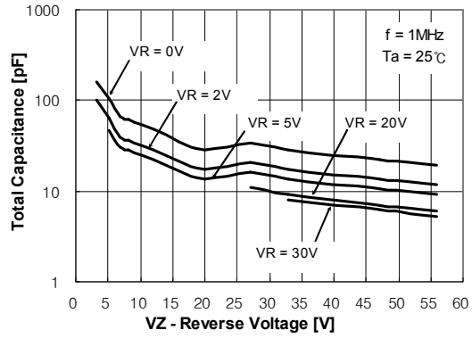
Figure 2. Total Capacitance
