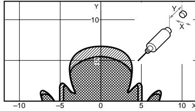
V600-D23P53 & V600-HS51 +V600-HA51
