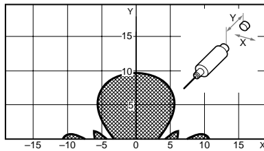
V600-D23P55 & V600-HS51 +V600-HA51
