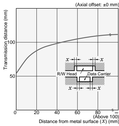
V600-D8KF04 Combined with V600-H07
