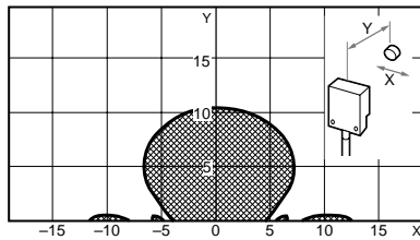
V600-D23P55 & V600-HS61 +V600-HA51
