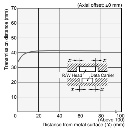
V600-D8KF04 Combined with V600-H11
