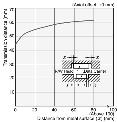
V600-D8KF04 Combined with V600-H07
