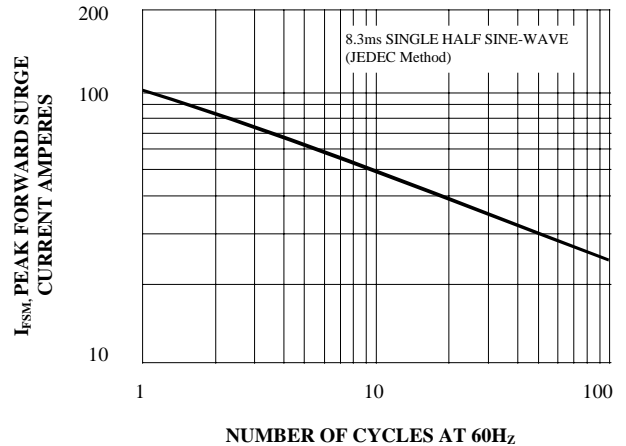
FIG. 7 - MAXIMUM NON-REPETITIVE FORWARD SURGE CURRENT UNIDIRECTIONAL
