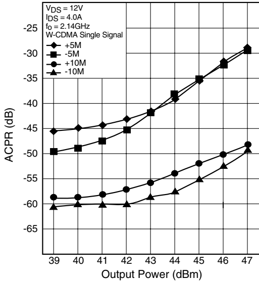
ACPR vs. OUTPUT POWER
