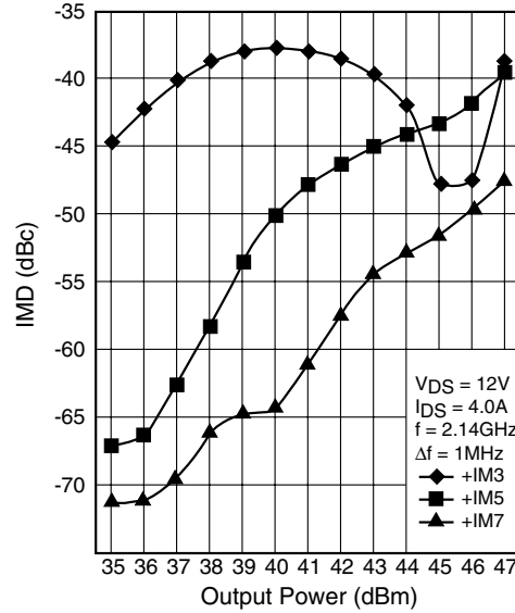
IMD vs. OUTPUT POWER
