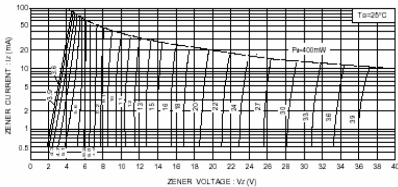
Fig.1 Zener characteristics
