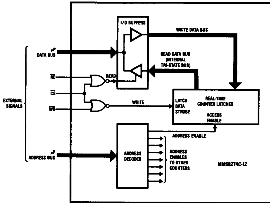
FIGURE 5. MM58274C-12 Microprocessor Interface Diagram
