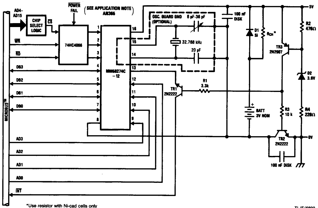
FIGURE 3. Typical System Connection Diagram
