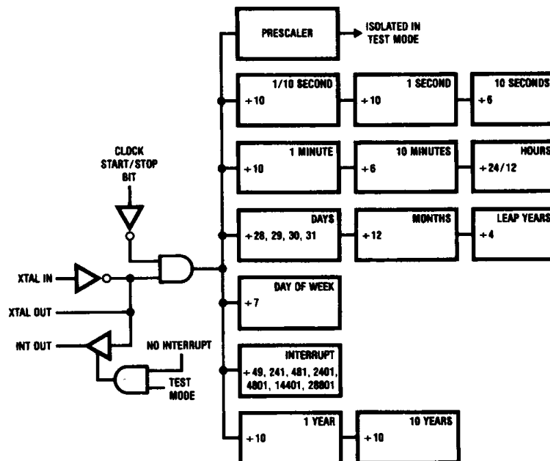
FIGURE 4. Test Mode Organization
