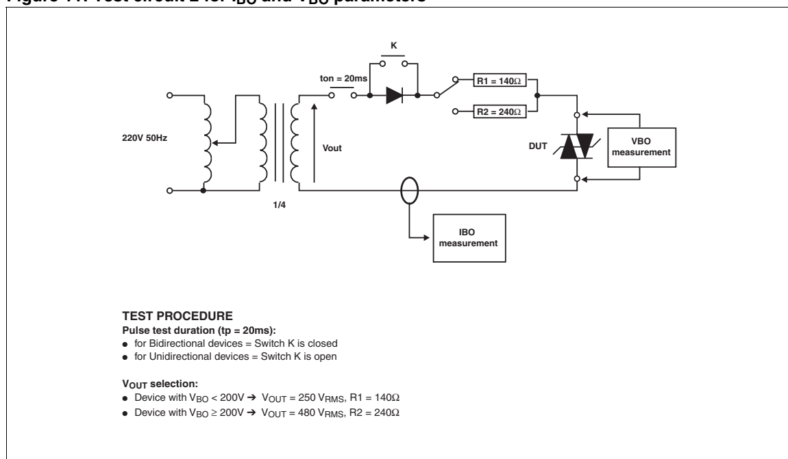
Figure 11: Test circuit 2 for I_{BO} and V_{BO} parameters
