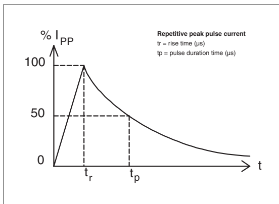
Figure 2: Pulse waveform
