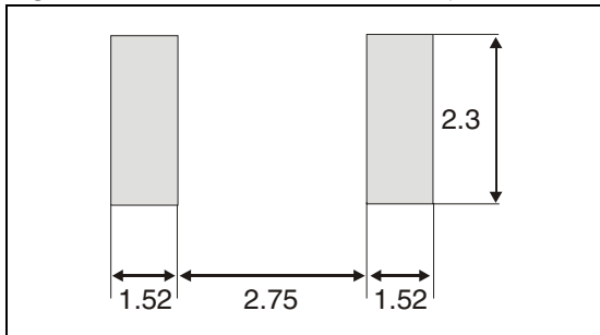
Figure 14: Foot Print Dimensions (in millimeters)
