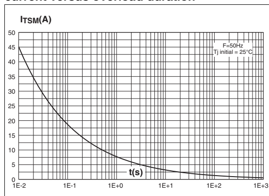
Figure 3: Non repetitive surge peak on-state current versus overload duration
