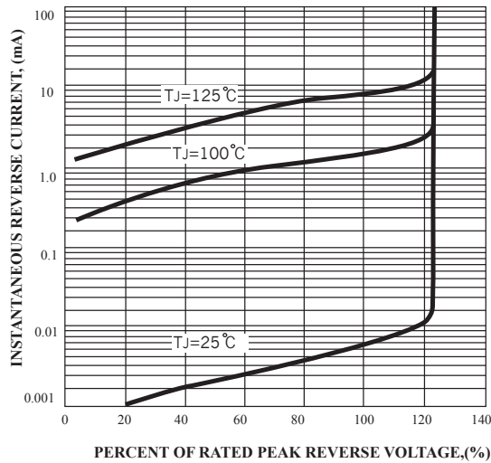
FIG.5-TYPICAL REVERSE CHARACTERISTICS
