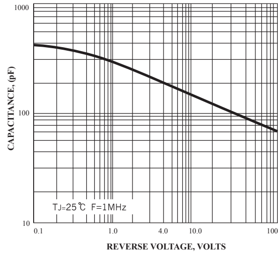
FIG.4-TYPICAL JUNCTION CAPACITANCE
