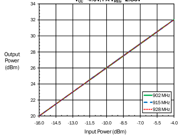
Input Power versus Output Power (Over Frequency) V_{CC}=4.0V, PA V_{REG}=2.85V
