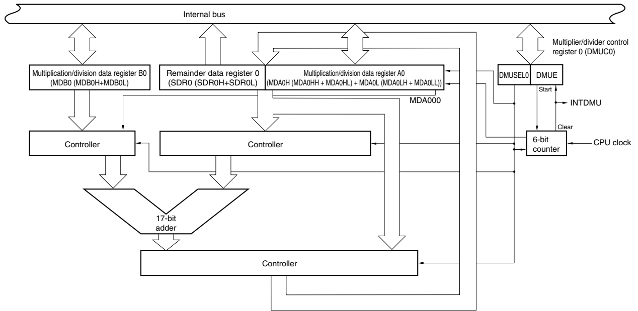
Figure 18-1. Block Diagram of Multiplier/Divider
