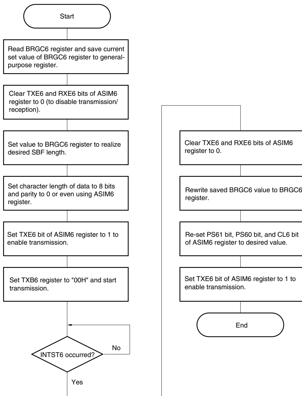
Figure 15-23. SBF Transmission
