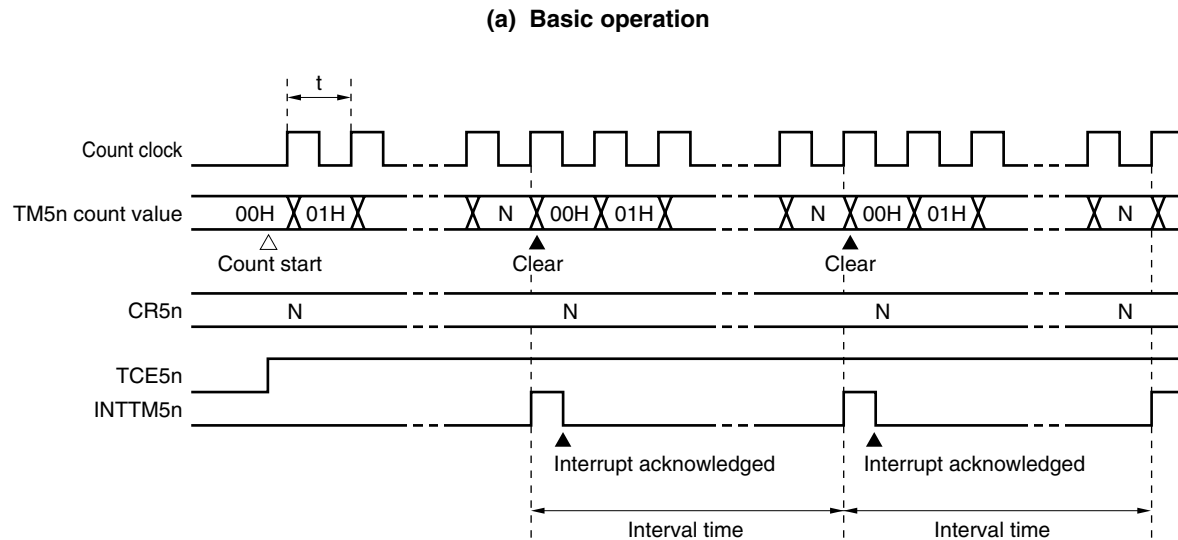
Figure 8-11. Interval Timer Operation Timing (1/2)
