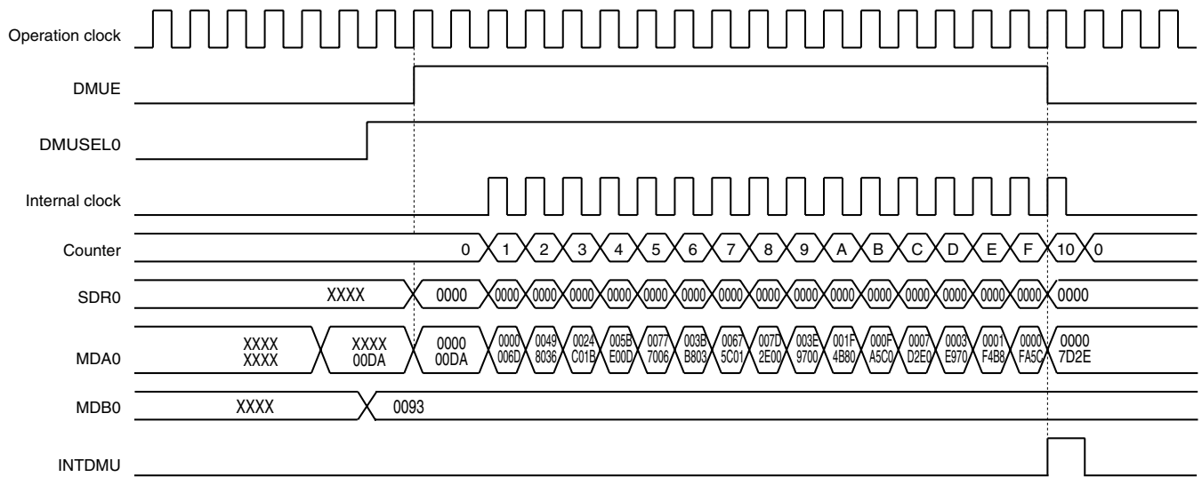
Figure 18-6. Timing Chart of Multiplication Operation (00DAH × 0093H)
