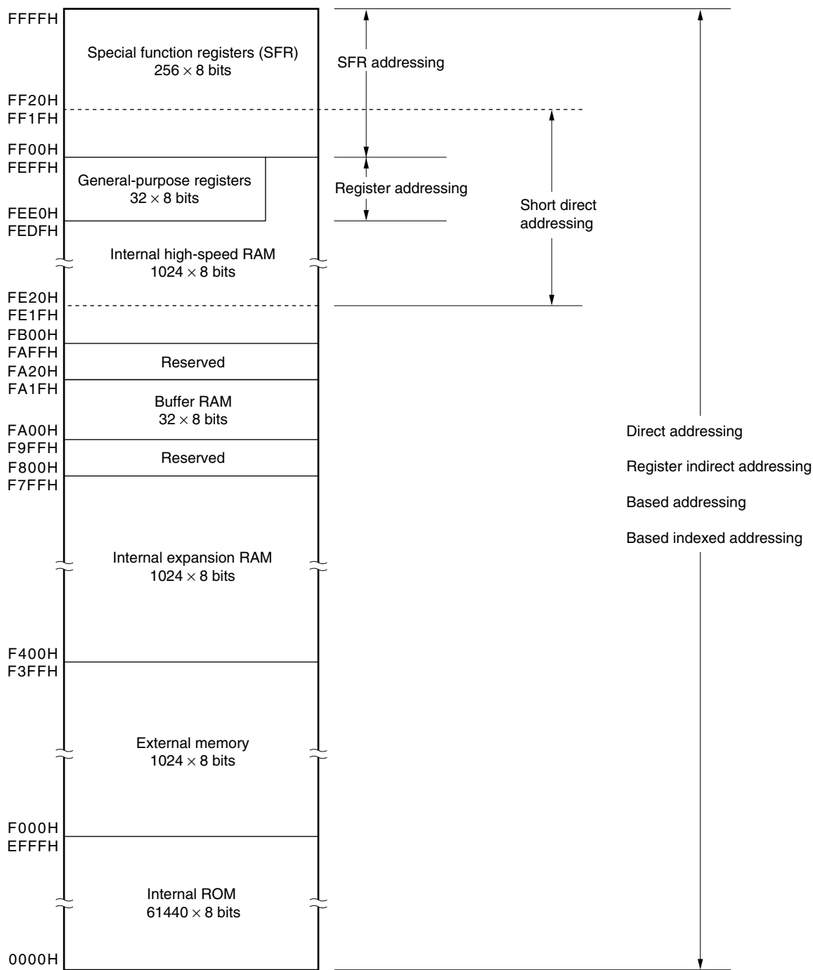
Figure 3-9. Correspondence Between Data Memory and Addressing ( \mu PD780148)
