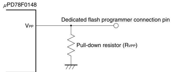
Figure 28-14. Example of Connection of V_{PP} Pin
