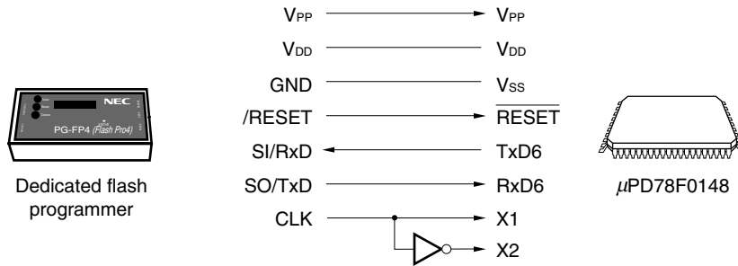
Figure 28-13. Communication with Dedicated Flash Programmer (UART6)
