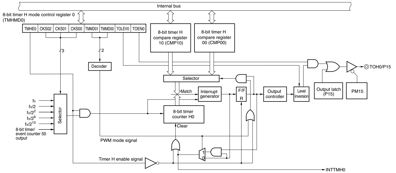
Figure 9-1. Block Diagram of 8-Bit Timer H0
