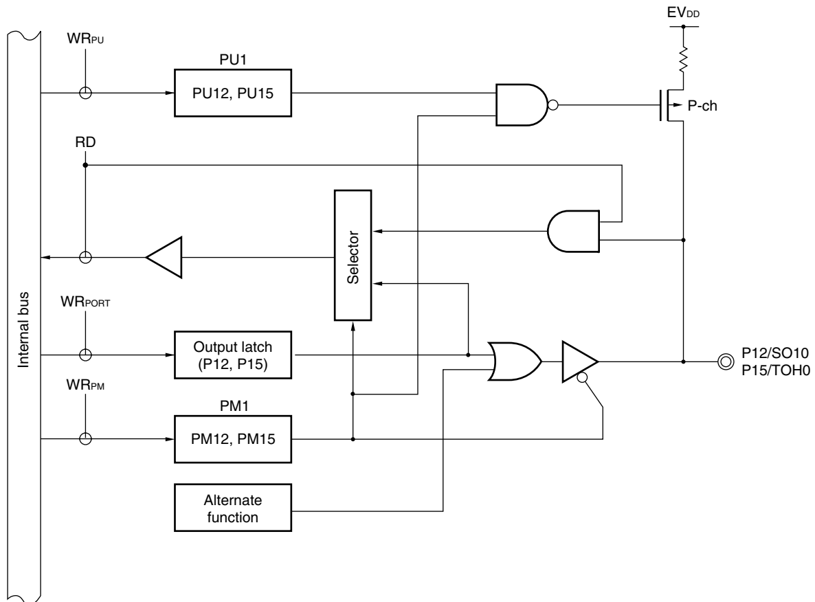
Figure 4-8. Block Diagram of P12 and P15
