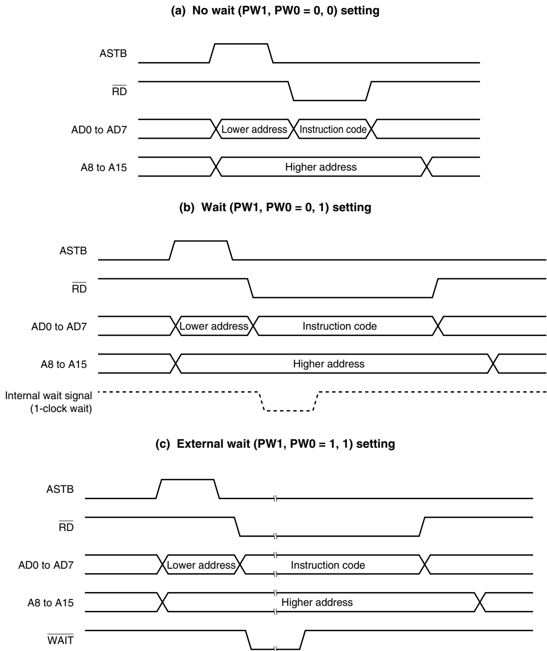
Figure 5-5. Instruction Fetch from External Memory
