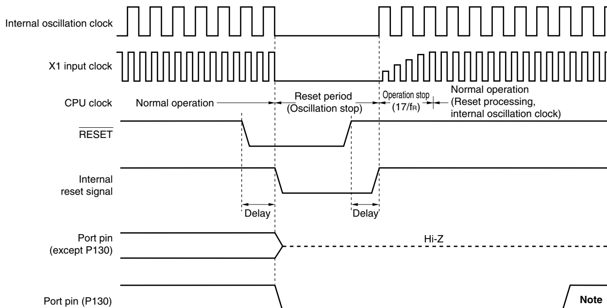
★ Figure 22-2. Timing of Reset by RESET Input
