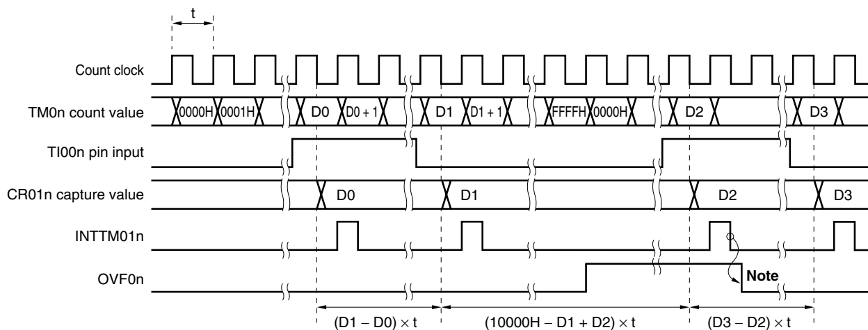
Figure 7-24. Timing of Pulse Width Measurement Operation with Free-Running Counter and One Capture Register (with Both Edges Specified)
