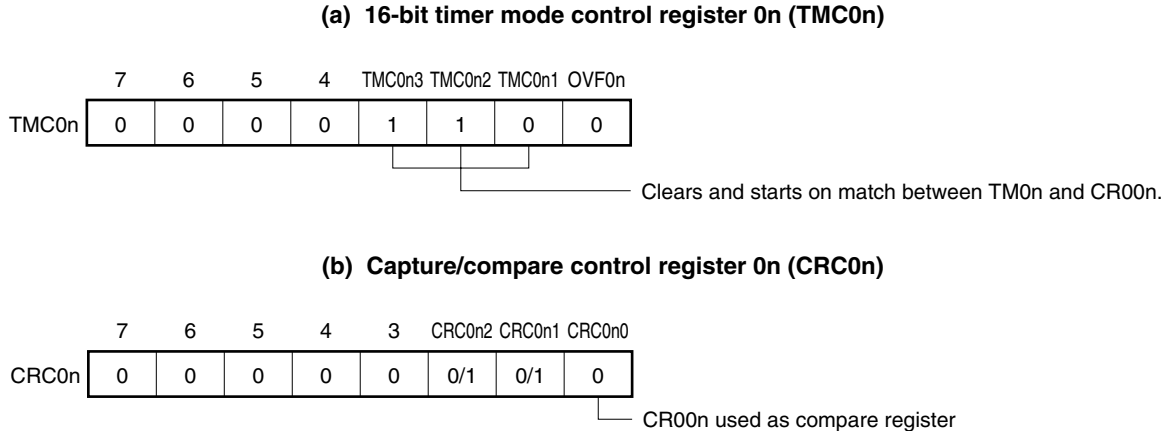
Figure 7-34. Control Register Settings in Square-Wave Output Mode (1/2)
