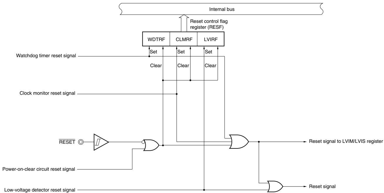
★ Figure 22-1. Block Diagram of Reset Function
