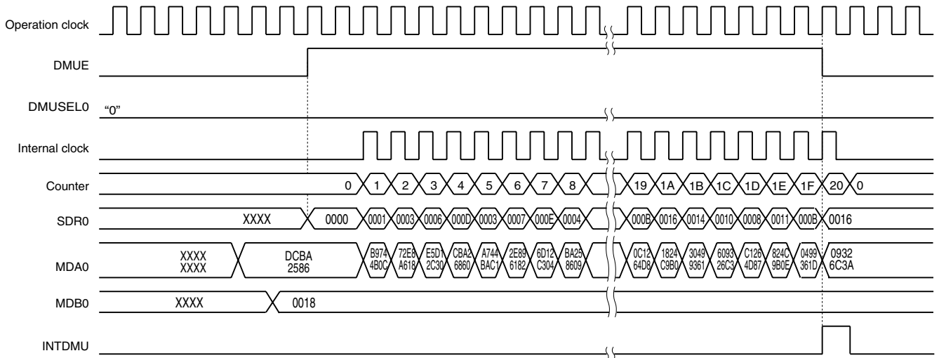
Figure 18-7. Timing Chart of Division Operation (DCBA2586H + 0018H)
