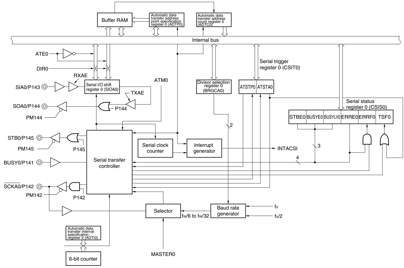
Figure 17-1. Block Diagram of Serial Interface CSIA0
