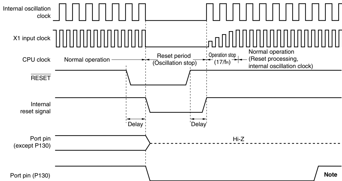
Figure 19-2. Timing of Reset by RESET Input
