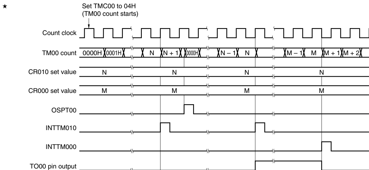
Figure 6-32. Timing of One-Shot Pulse Output Operation with Software Trigger
