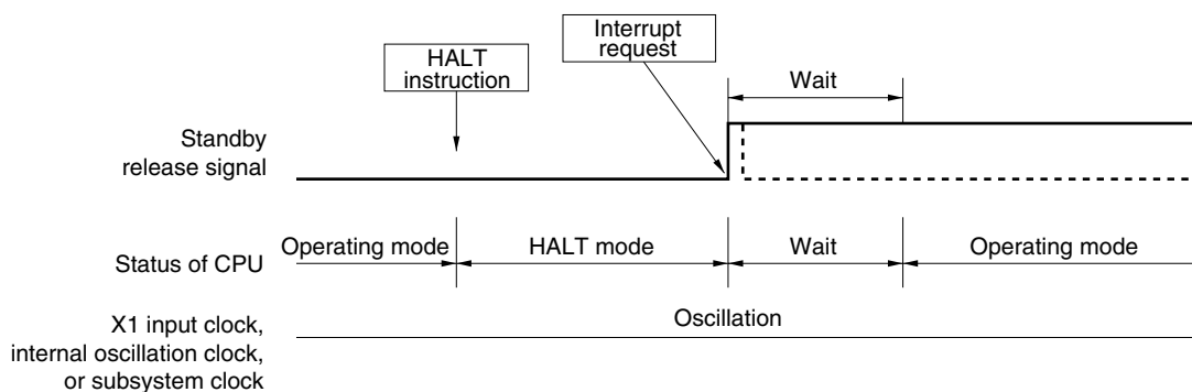
Figure 18-3. HALT Mode Release by Interrupt Request Generation
