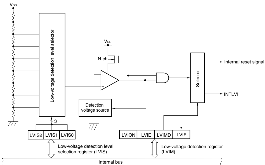
Figure 22-1. Block Diagram of Low-Voltage Detector
