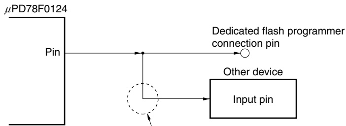
Figure 25-15. Malfunction of Other Device
