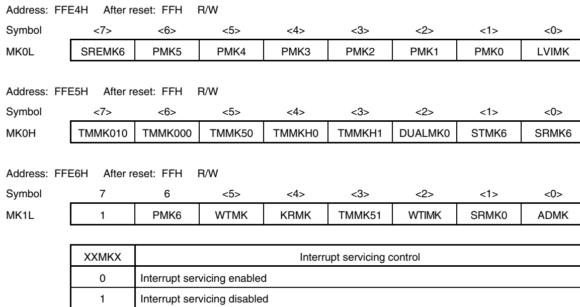
Figure 16-3. Format of Interrupt Mask Flag Registers (MK0L, MK0H, MK1L)
