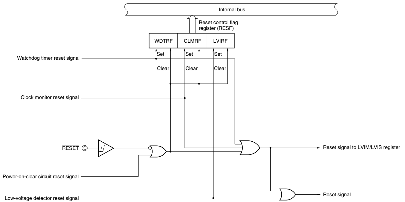
Figure 16-1. Block Diagram of Reset Function
