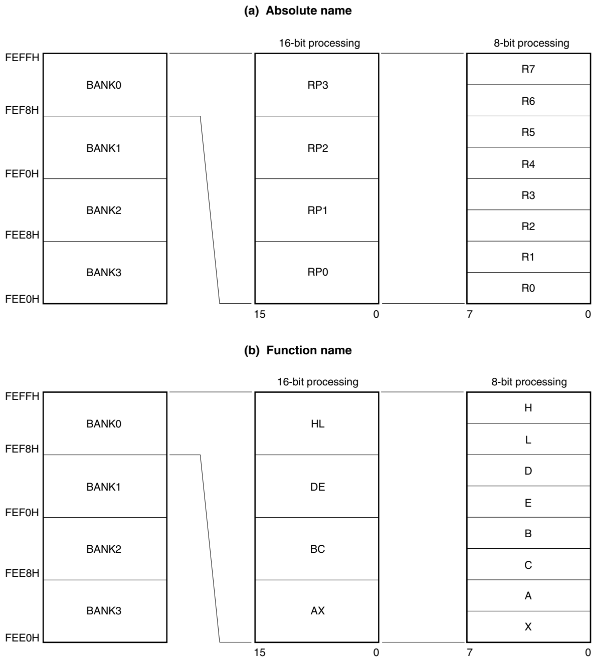
Figure 3-12. Configuration of General-Purpose Registers
