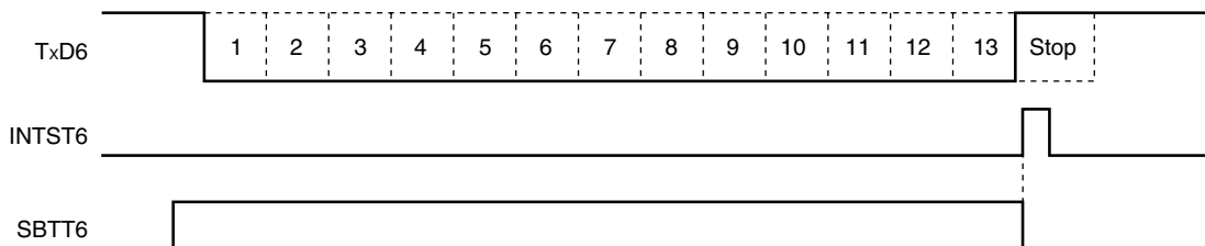
Figure 12-22. SBF Transmission
