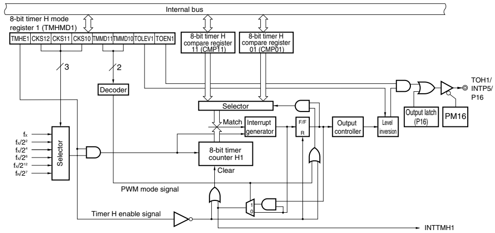
Figure 8-2. Block Diagram of 8-Bit Timer H1
