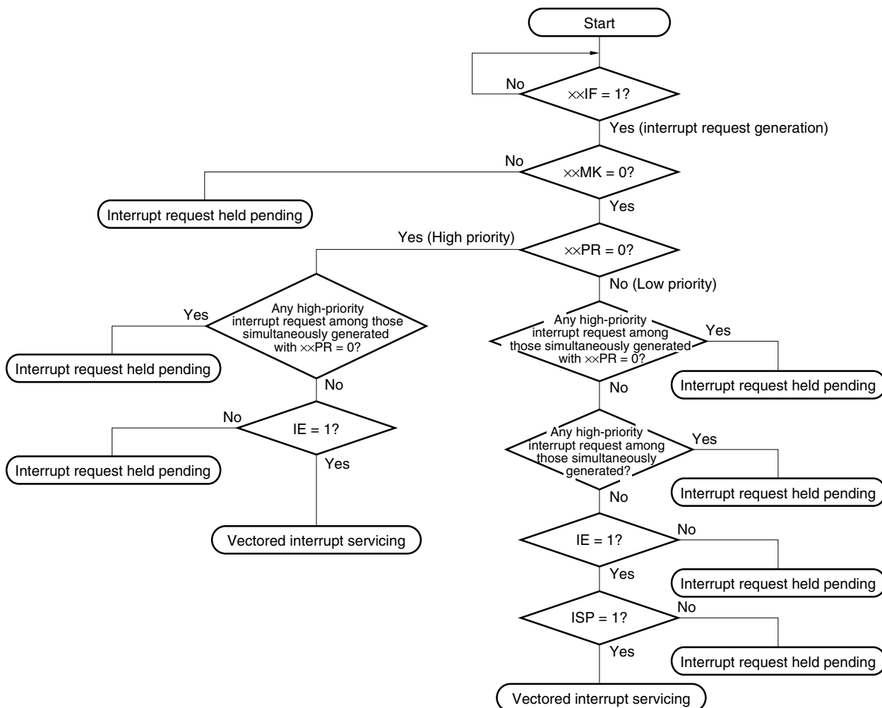
Figure 14-7. Interrupt Request Acknowledgment Processing Algorithm
