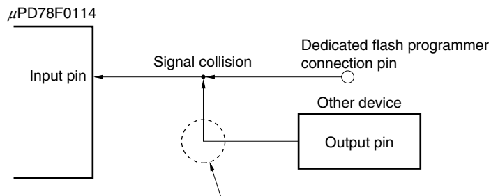
Figure 23-14. Signal Collision (Input Pin of Serial Interface)
