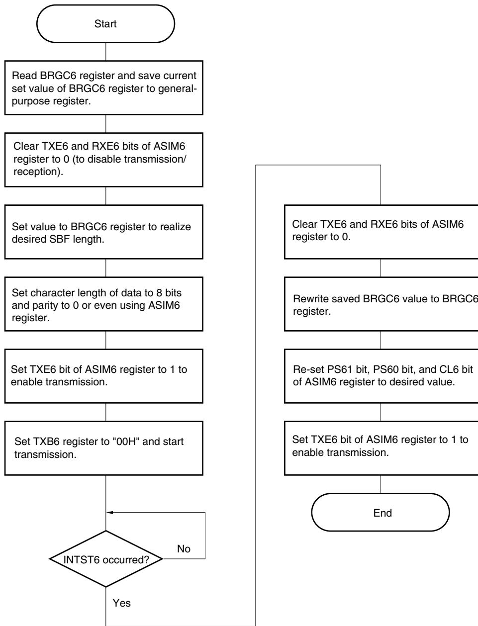
Figure 13-23. SBF Transmission
