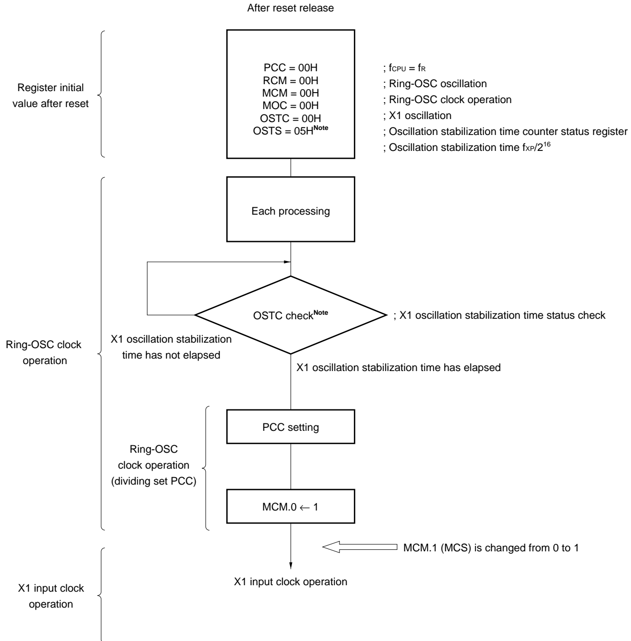
Figure 5-14. Switching from Ring-OSC Clock to X1 Input Clock (Flowchart)
