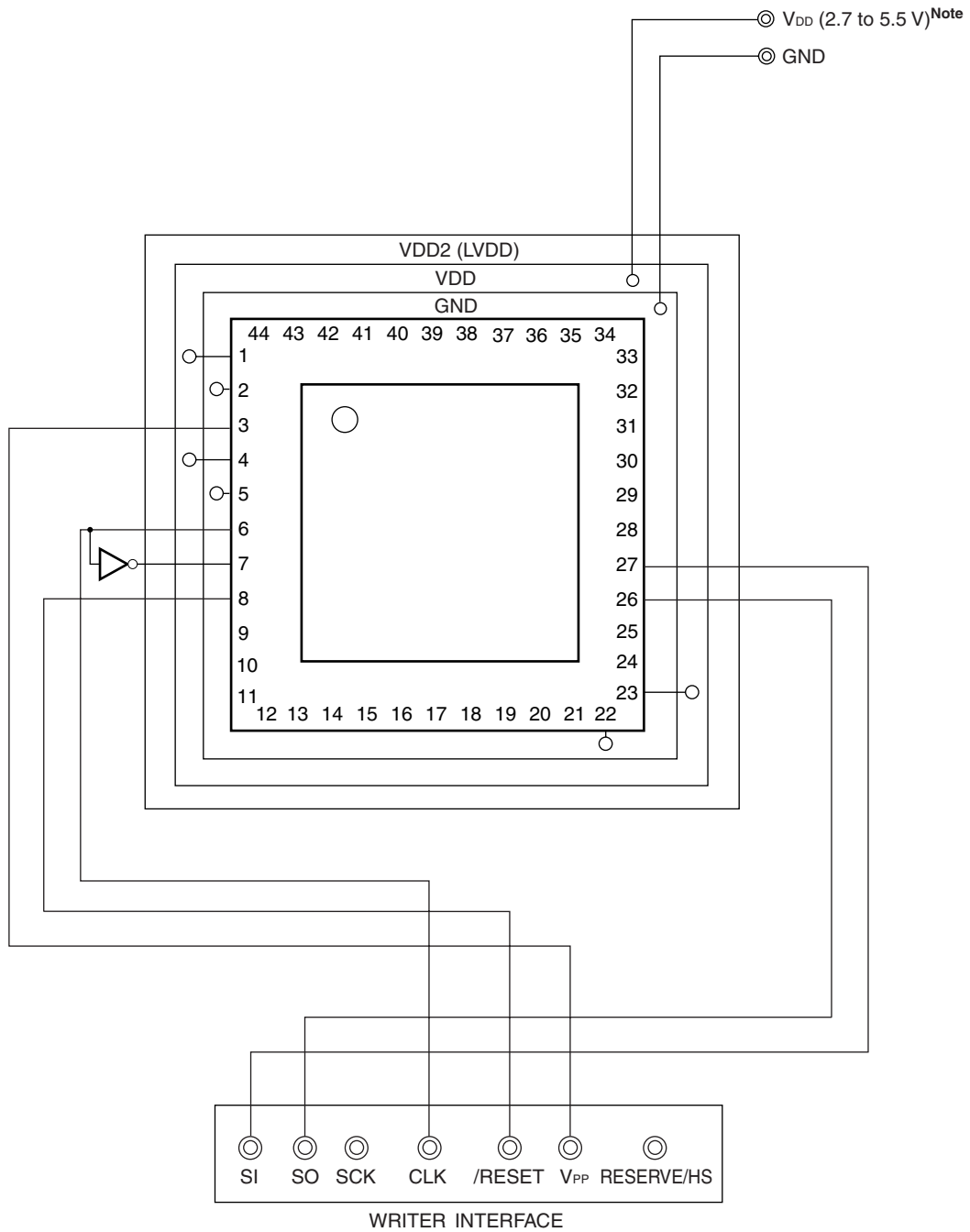
Figure 23-6. Example of Wiring Adapter for Flash Memory Writing in UART (UART6) Mode
