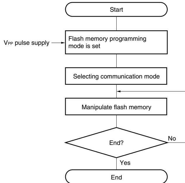
Figure 23-17. Flash Memory Manipulation Procedure
