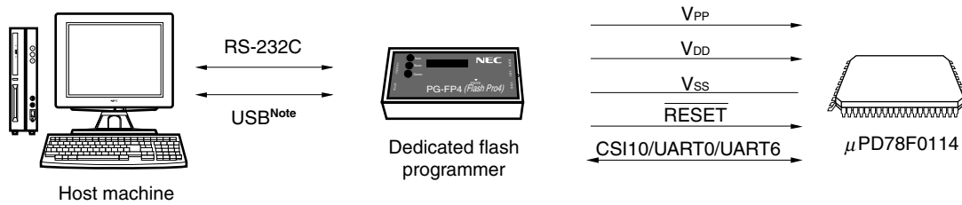
Figure 23-7. Environment for Writing Program to Flash Memory
