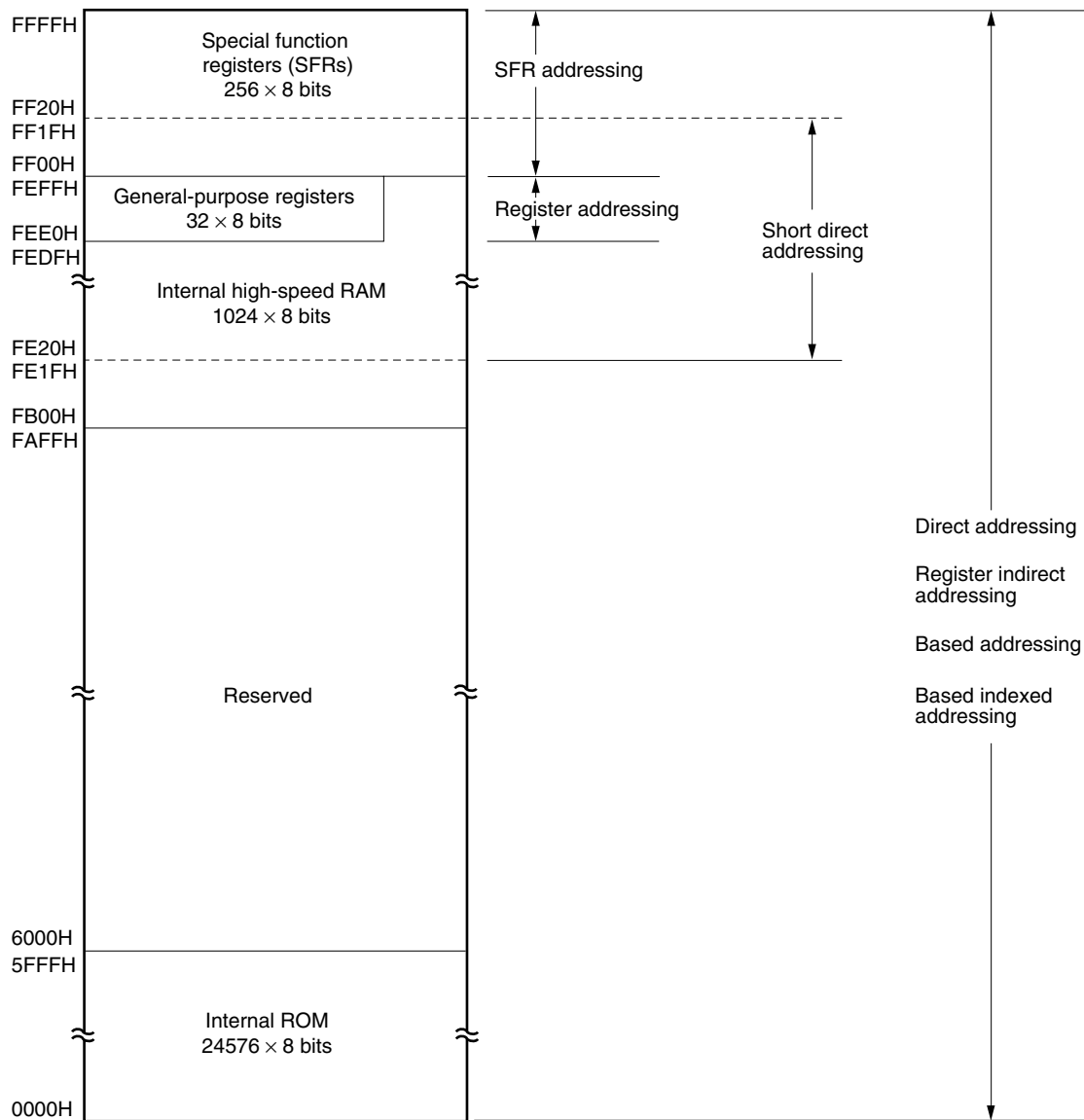
Figure 3-8. Correspondence Between Data Memory and Addressing ( \mu PD780113)
