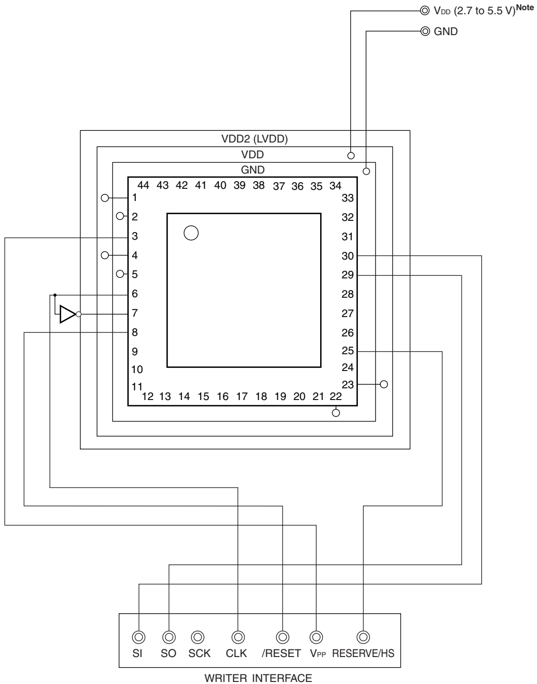
Figure 23-5. Example of Wiring Adapter for Flash Memory Writing in UART (UART0 + HS) Mode
