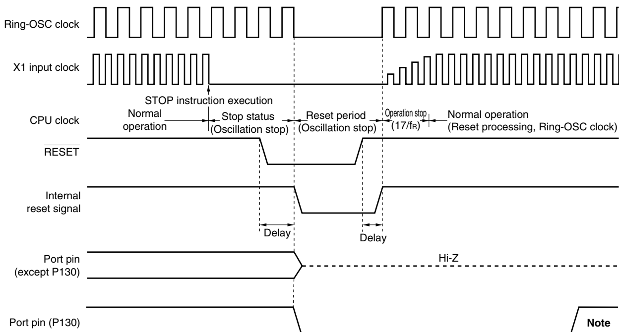
Figure 18-4. Timing of Reset in STOP Mode by RESET Input
