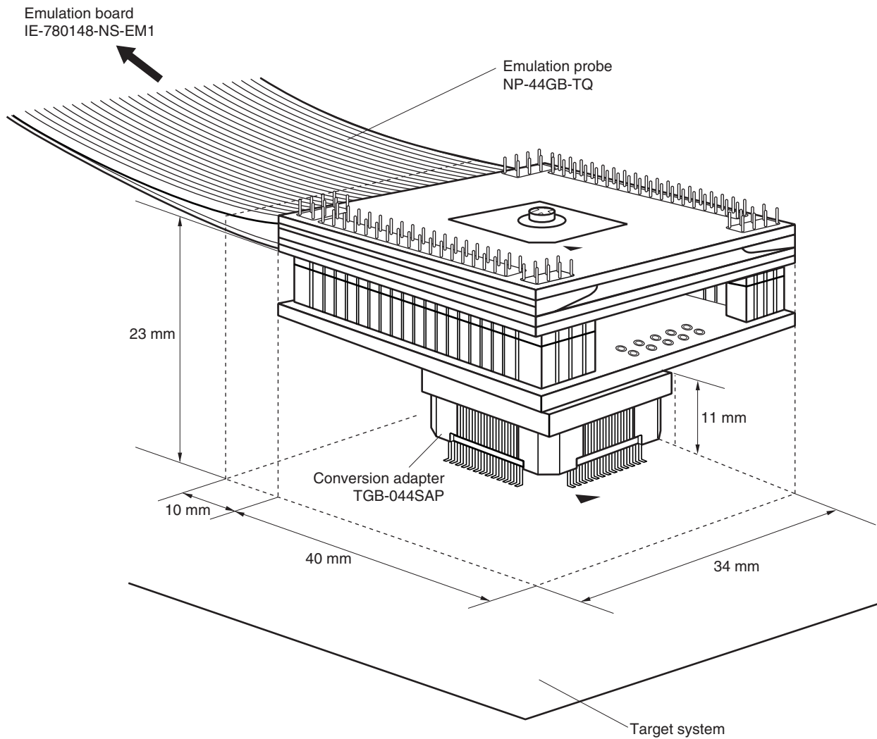
Figure B-2. Connection Conditions of Target System
