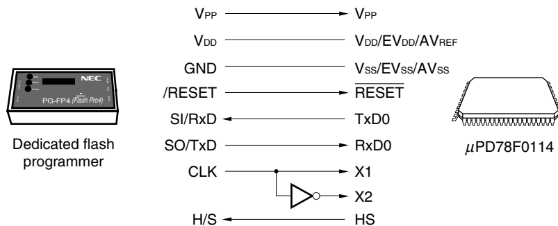
Figure 23-11. Communication with Dedicated Flash Programmer (UART0 + HS)
