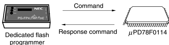
Figure 23-19. Communication Commands
