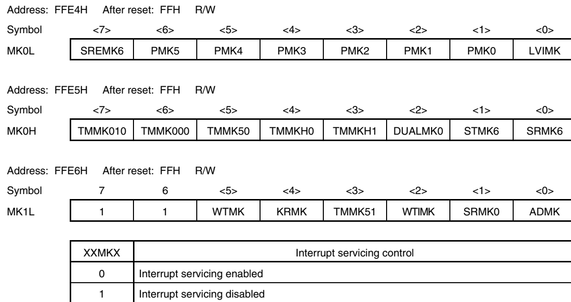
Figure 15-3. Format of Interrupt Mask Flag Registers (MK0L, MK0H, MK1L)
