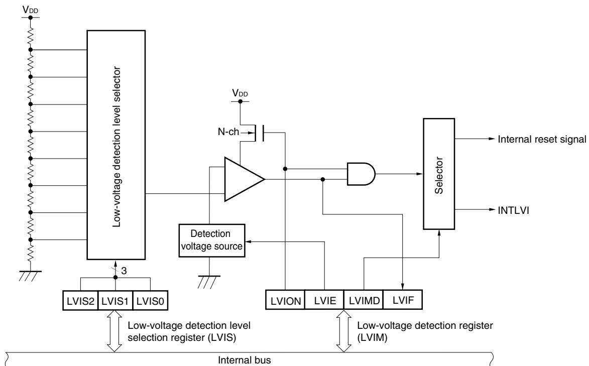
Figure 21-1. Block Diagram of Low-Voltage Detector
