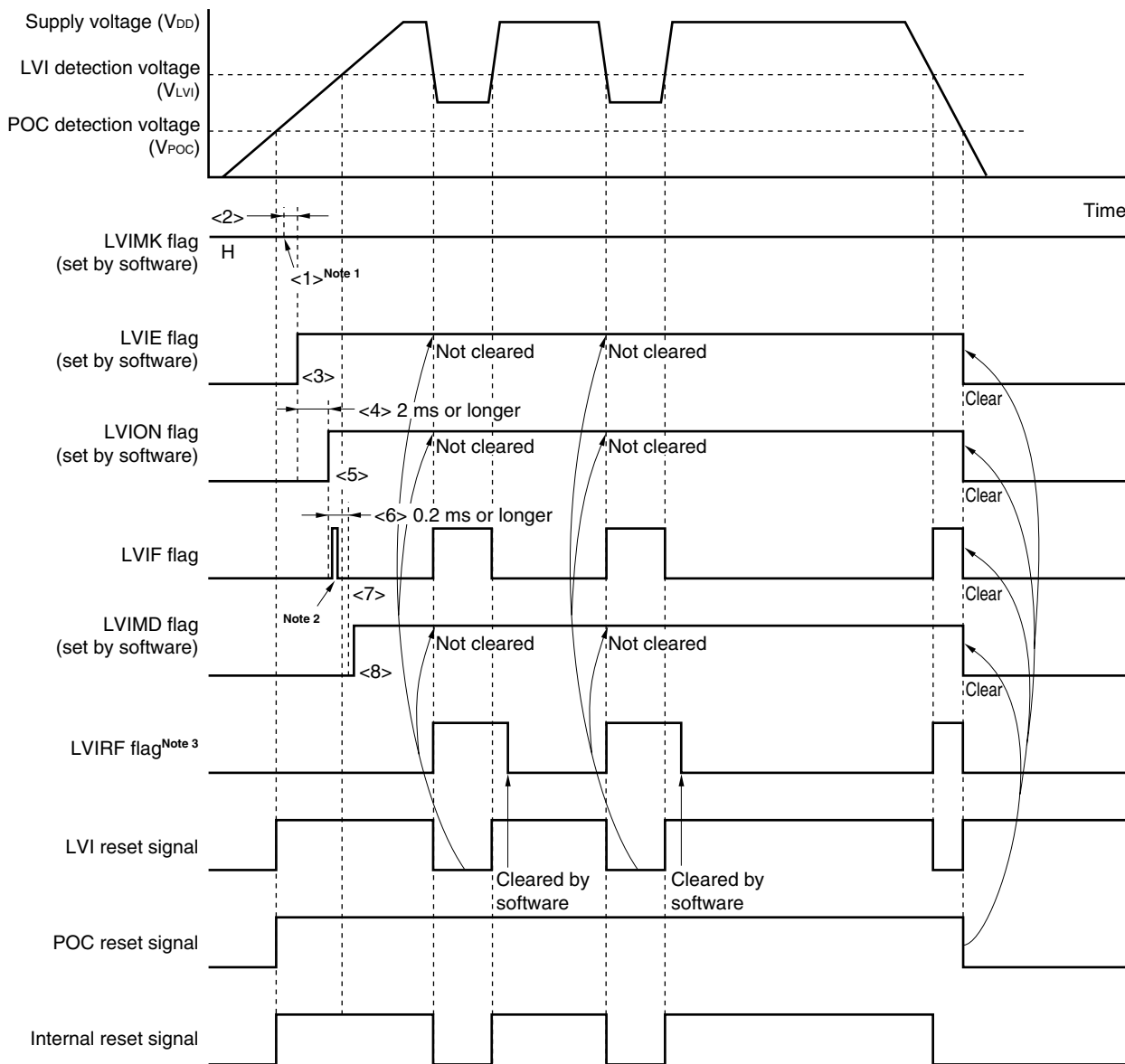
Figure 21-4. Timing of Low-Voltage Detector Internal Reset Signal Generation
