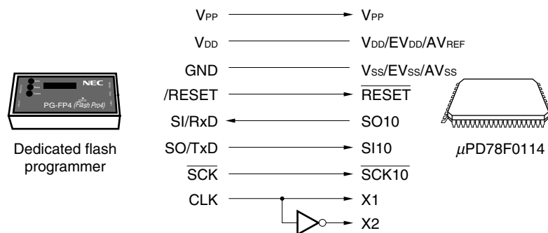
Figure 23-8. Communication with Dedicated Flash Programmer (CSI10)
