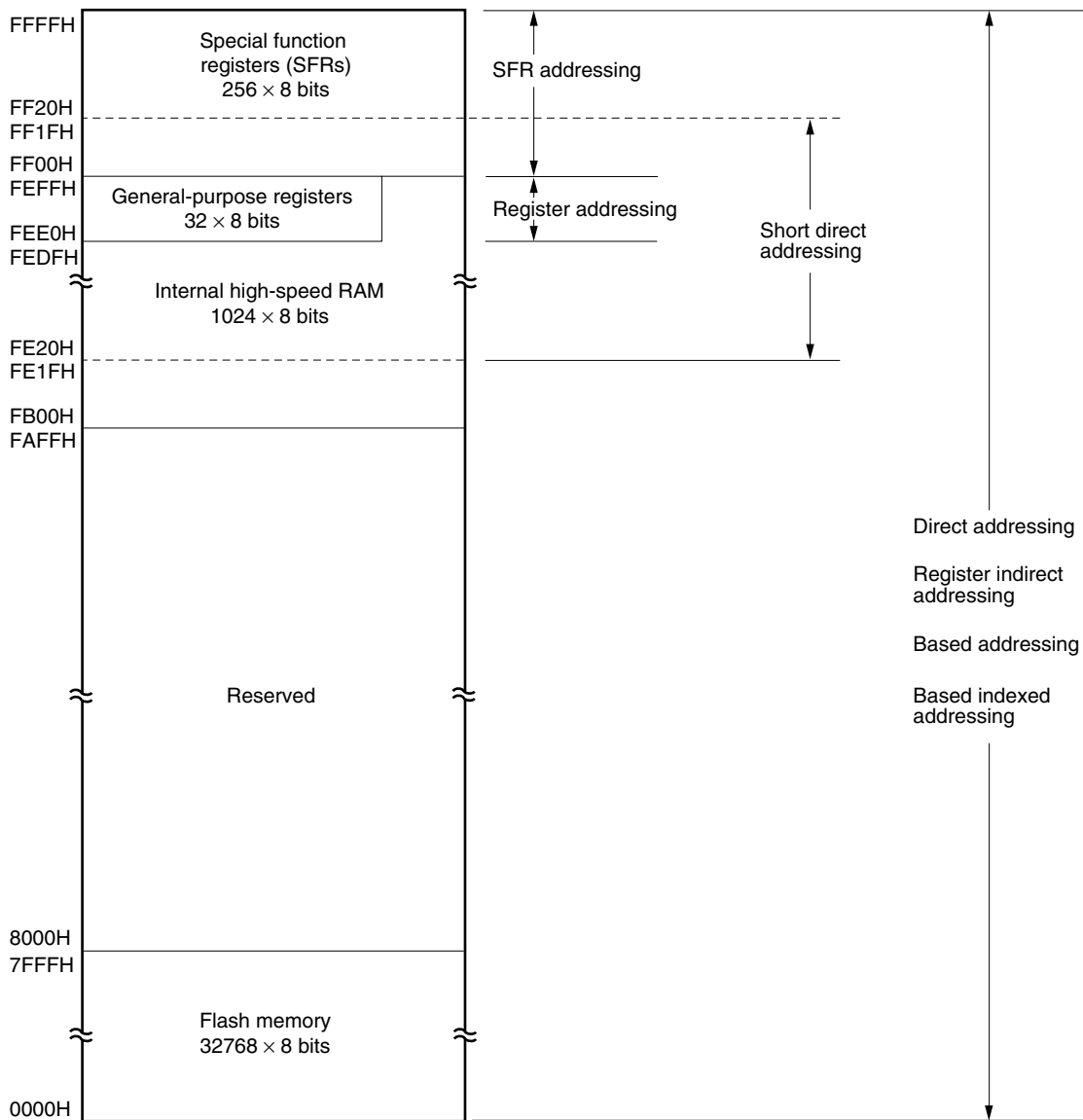
Figure 3-10. Correspondence Between Data Memory and Addressing ( \mu PD78F0114)
