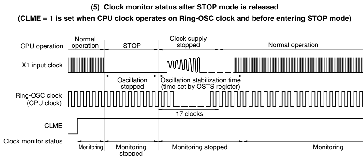
Figure 19-3. Timing of Clock Monitor (3/4)
