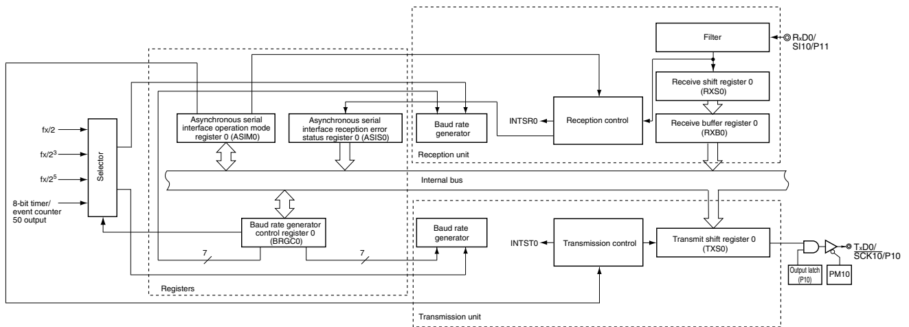
Figure 12-1. Block Diagram of Serial Interface UART0
