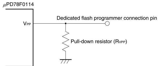
Figure 23-13. Example of Connection of V_{PP} Pin
