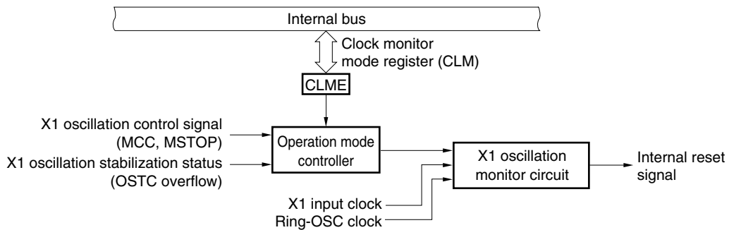
Figure 19-1. Block Diagram of Clock Monitor
