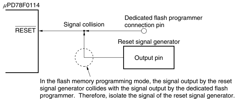
Figure 23-16. Signal Collision ( \overline{\text{RESET}} Pin)
