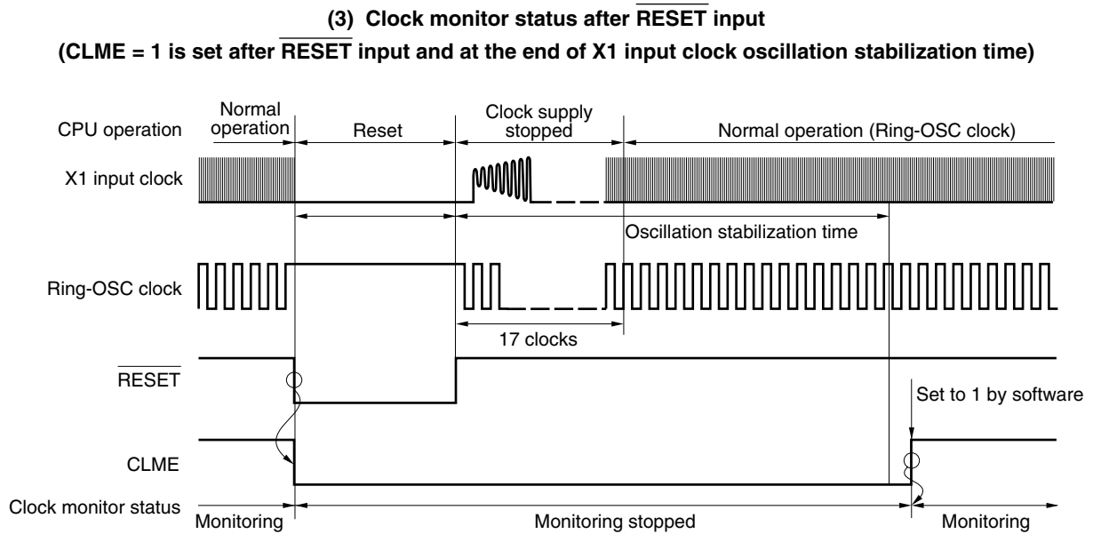
Figure 19-3. Timing of Clock Monitor (2/4)
