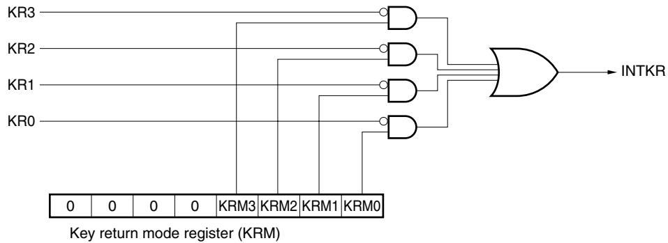
Figure 16-1. Block Diagram of Key Interrupt
