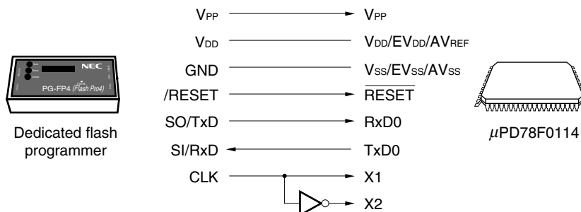
Figure 23-10. Communication with Dedicated Flash Programmer (UART0)
