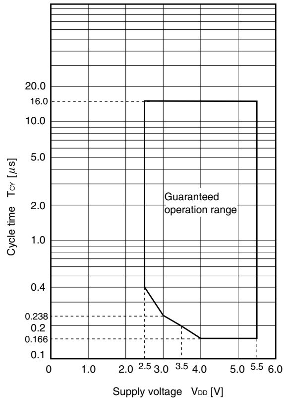
T_{CY} vs. V_{DD} (X1 Input Clock Operation)
