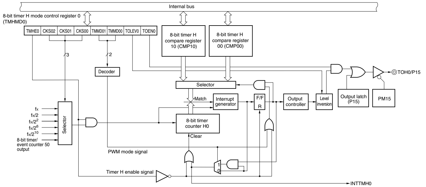
Figure 8-1. Block Diagram of 8-Bit Timer H0
