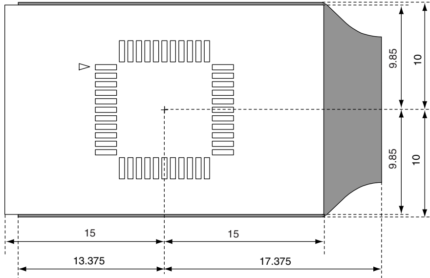
Figure B-3. Restricted Area on Target System
