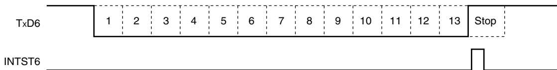
Figure 13-23. SBF Transmission
