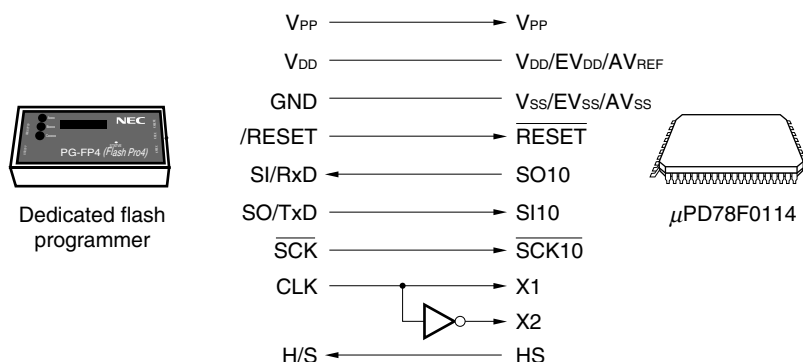
Figure 23-9. Communication with Dedicated Flash Programmer (CSI10 + HS)
