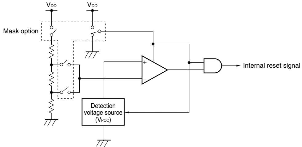
Figure 20-1. Block Diagram of Power-on-Clear Circuit
