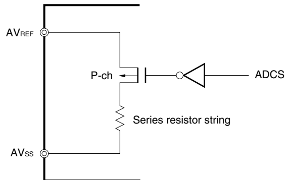
Figure 11-2. Circuit Configuration of Series Resistor String
