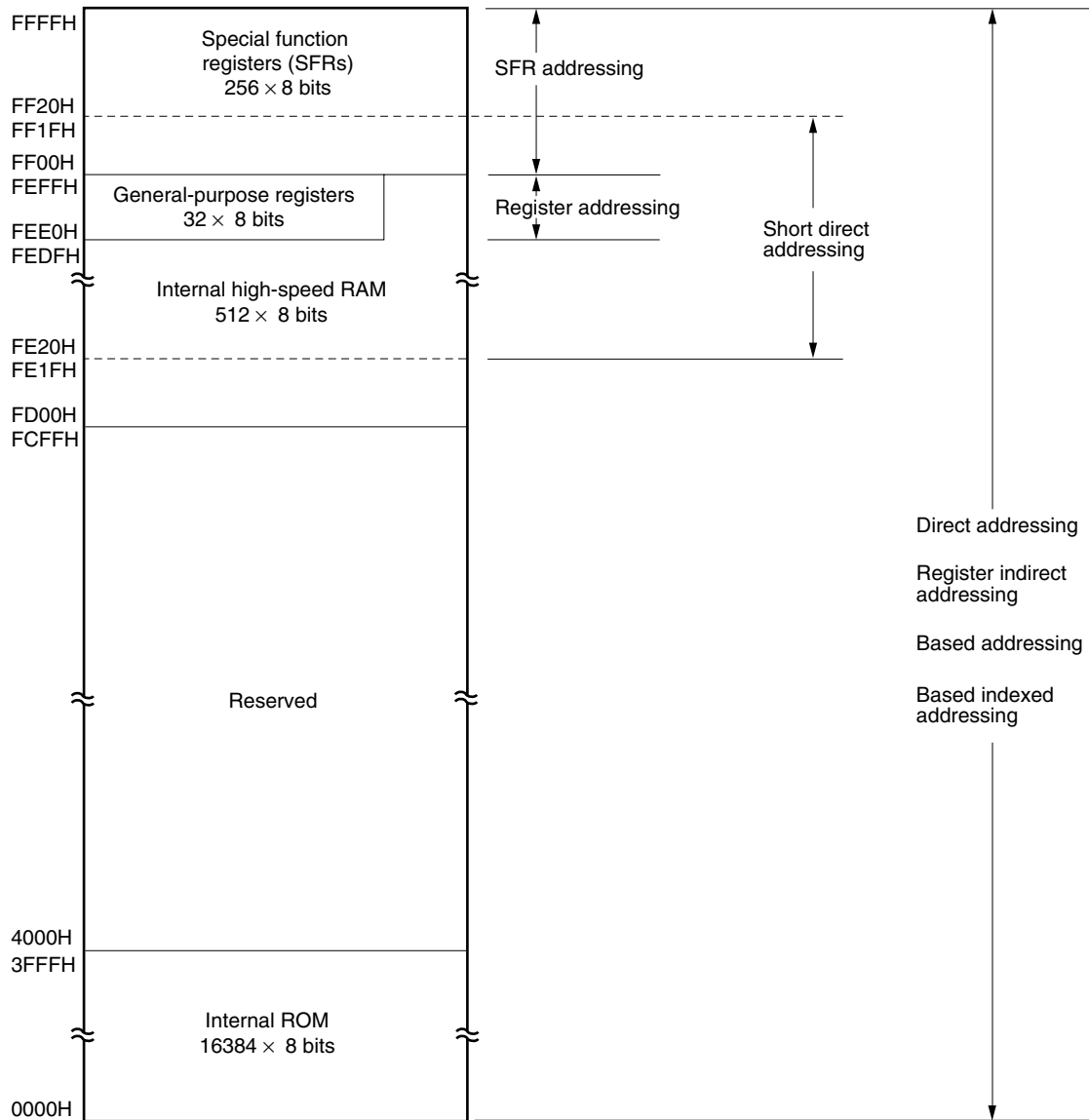
Figure 3-7. Correspondence Between Data Memory and Addressing ( \mu PD780112)
