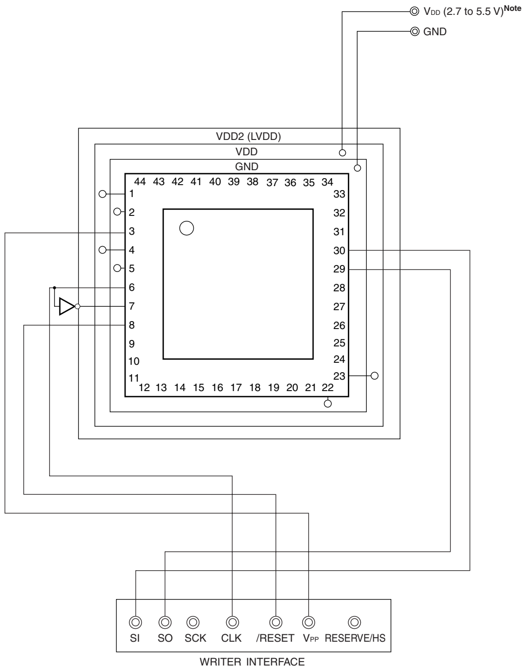
Figure 23-4. Example of Wiring Adapter for Flash Memory Writing in UART (UART0) Mode
