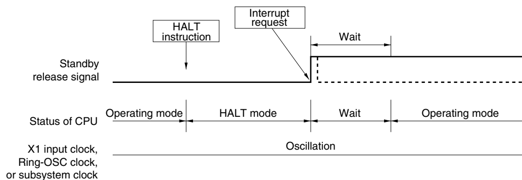
Figure 17-3. HALT Mode Release by Interrupt Request Generation
