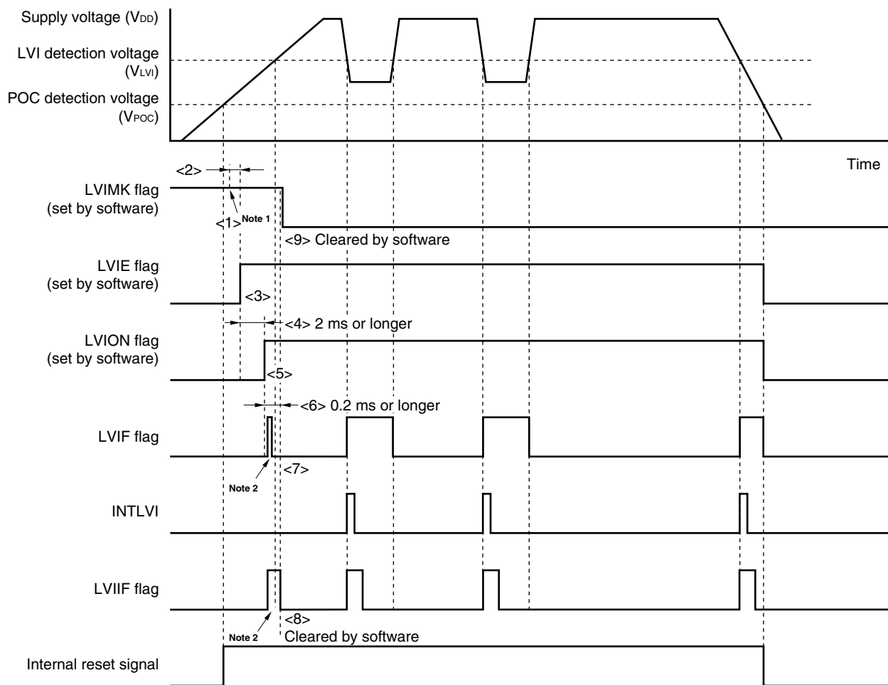
Figure 21-5. Timing of Low-Voltage Detector Interrupt Signal Generation
