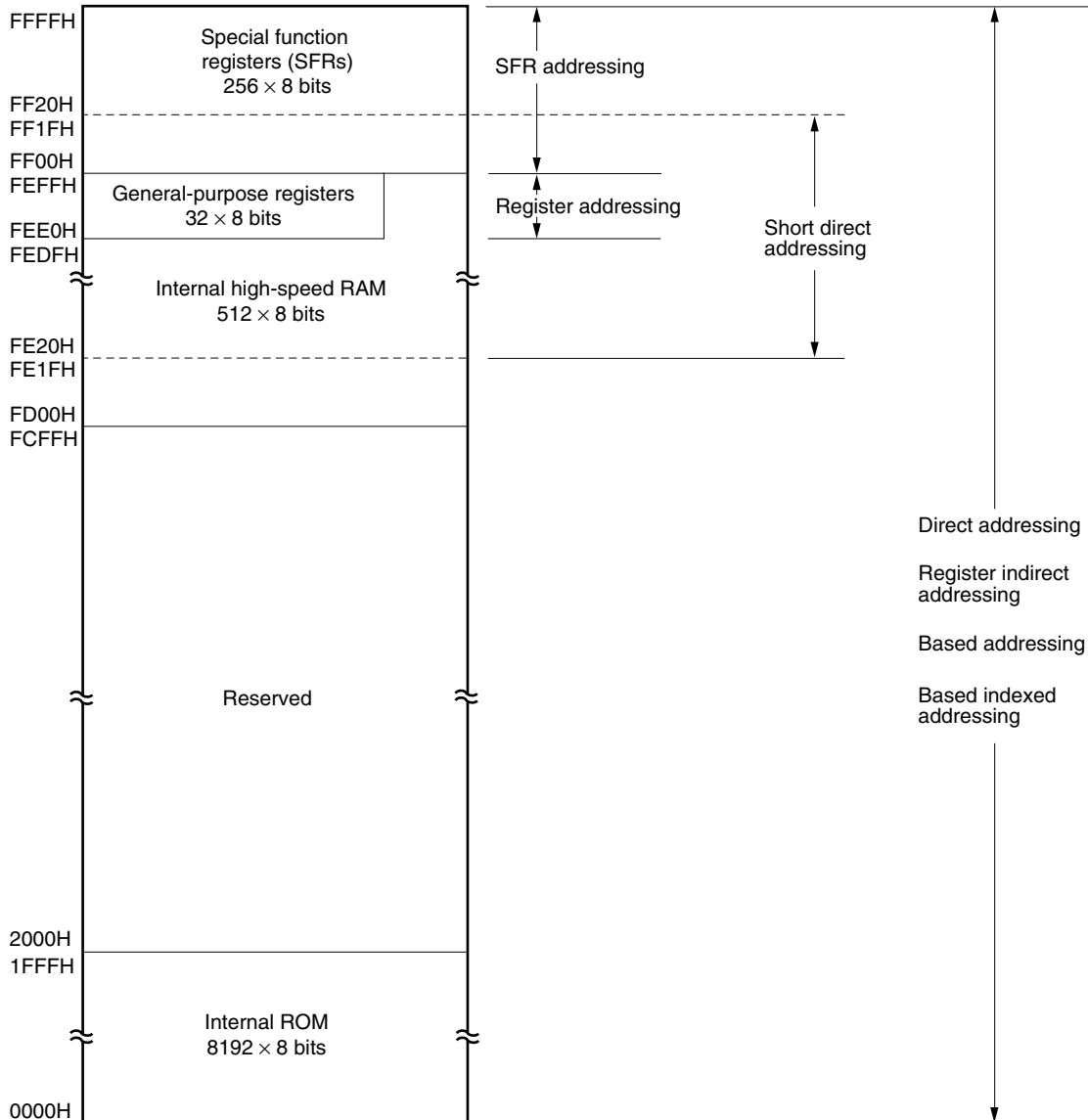
Figure 3-6. Correspondence Between Data Memory and Addressing ( \mu PD780111)
