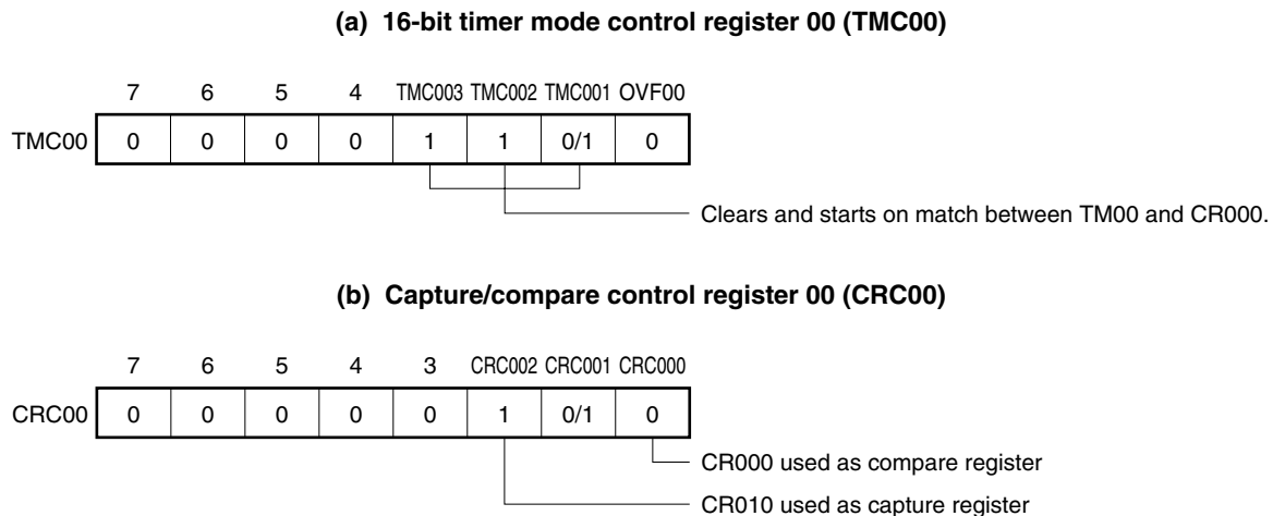
Figure 6-10. Control Register Settings for Interval Timer Operation (1/2)
