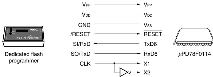
Figure 23-12. Communication with Dedicated Flash Programmer (UART6)
