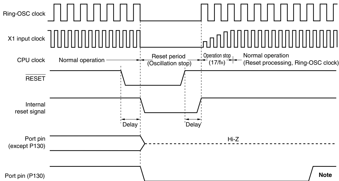
Figure 18-2. Timing of Reset by RESET Input
