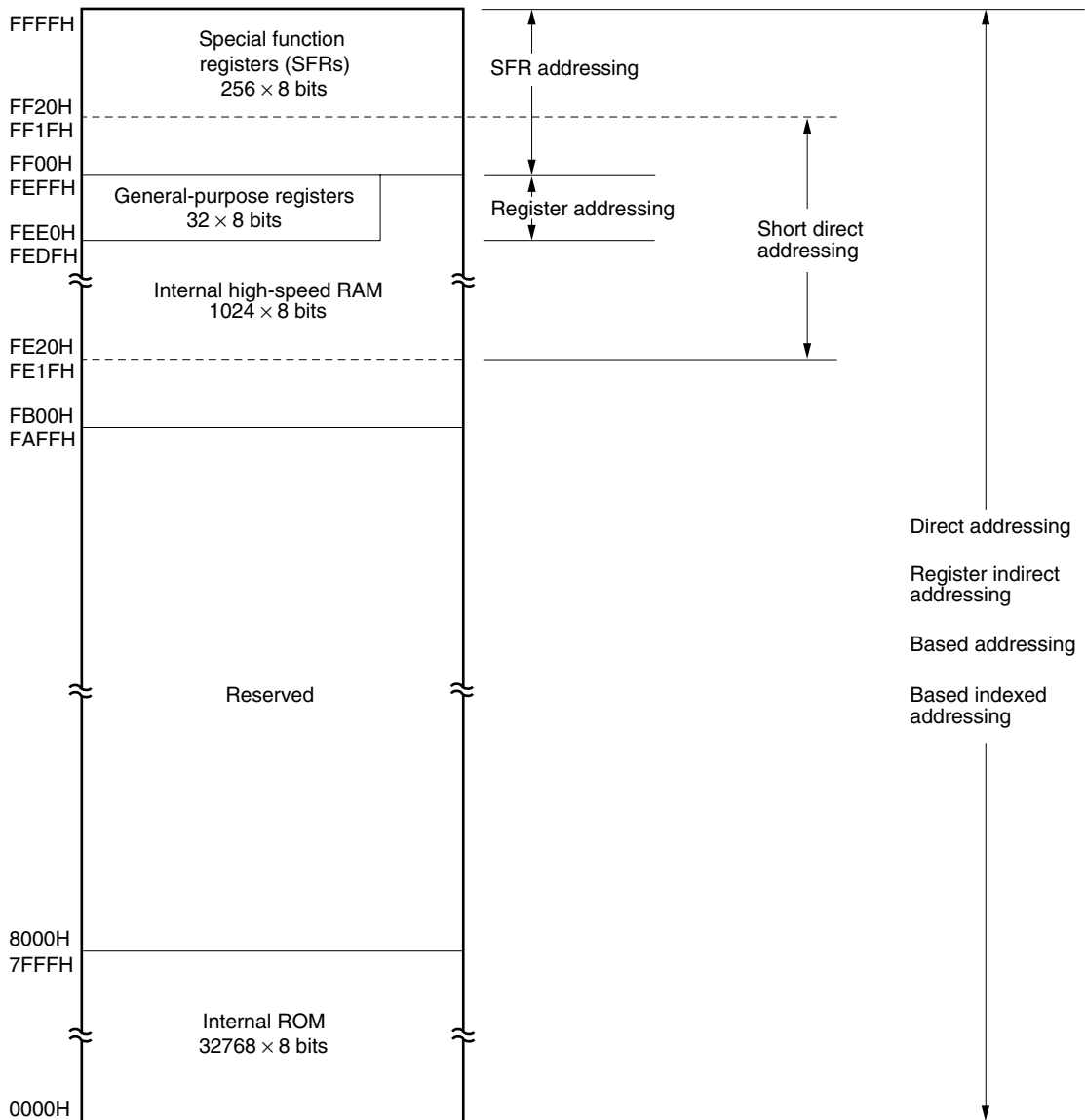
Figure 3-9. Correspondence Between Data Memory and Addressing ( \mu PD780114)
