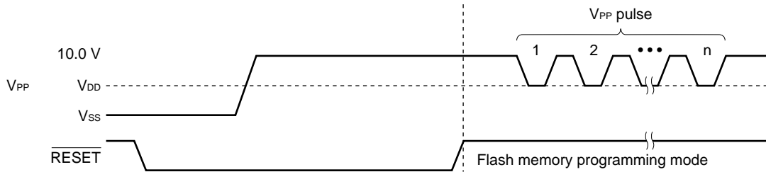
Figure 23-18. Flash Memory Programming Mode
