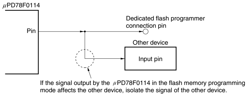
Figure 23-15. Malfunction of Other Device
