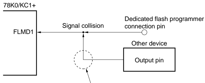
Figure 23-11. Signal Collision (Input Pin of Serial Interface)
