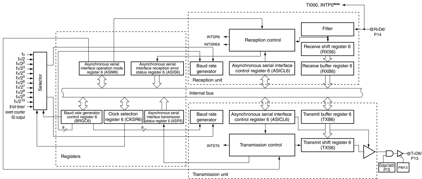
Figure 13-4. Block Diagram of Serial Interface UART6
