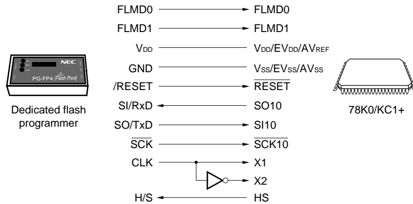
Figure 23-7. Communication with Dedicated Flash Programmer (CSI10 + HS)
