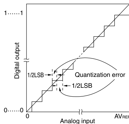
Figure 11-14. Quantization Error
