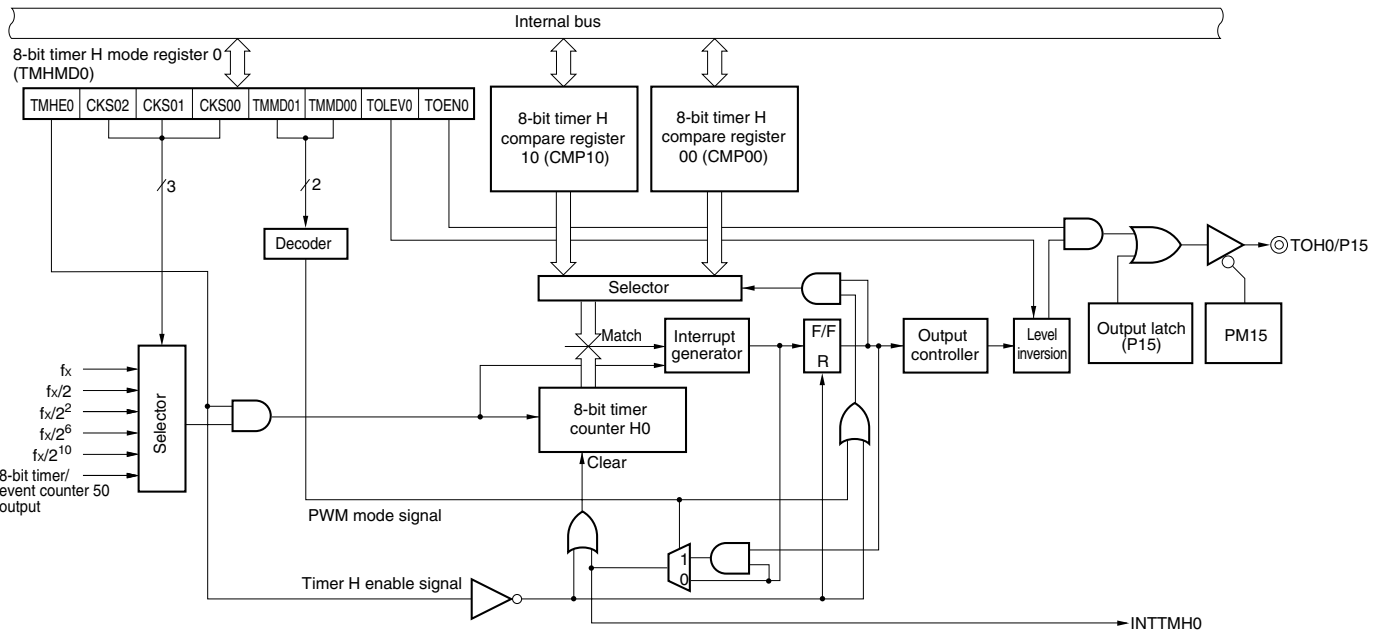
Figure 8-1. Block Diagram of 8-Bit Timer H0
