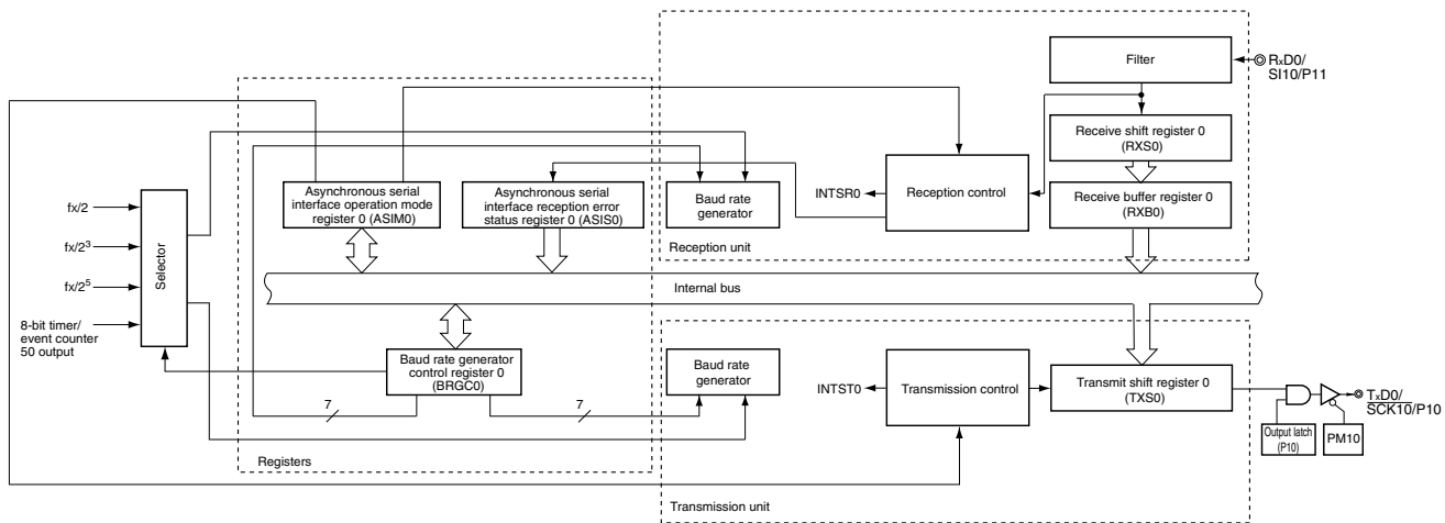
Figure 12-1. Block Diagram of Serial Interface UART0
