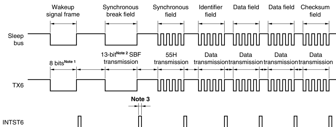
Figure 13-1. LIN Transmission Operation
