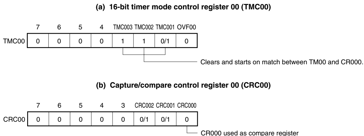
Figure 6-26. Control Register Settings in External Event Counter Mode (with Rising Edge Specified) (1/2)
