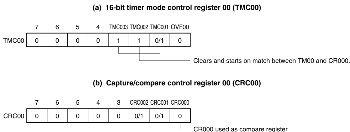
Figure 6-10. Control Register Settings for Interval Timer Operation (1/2)
