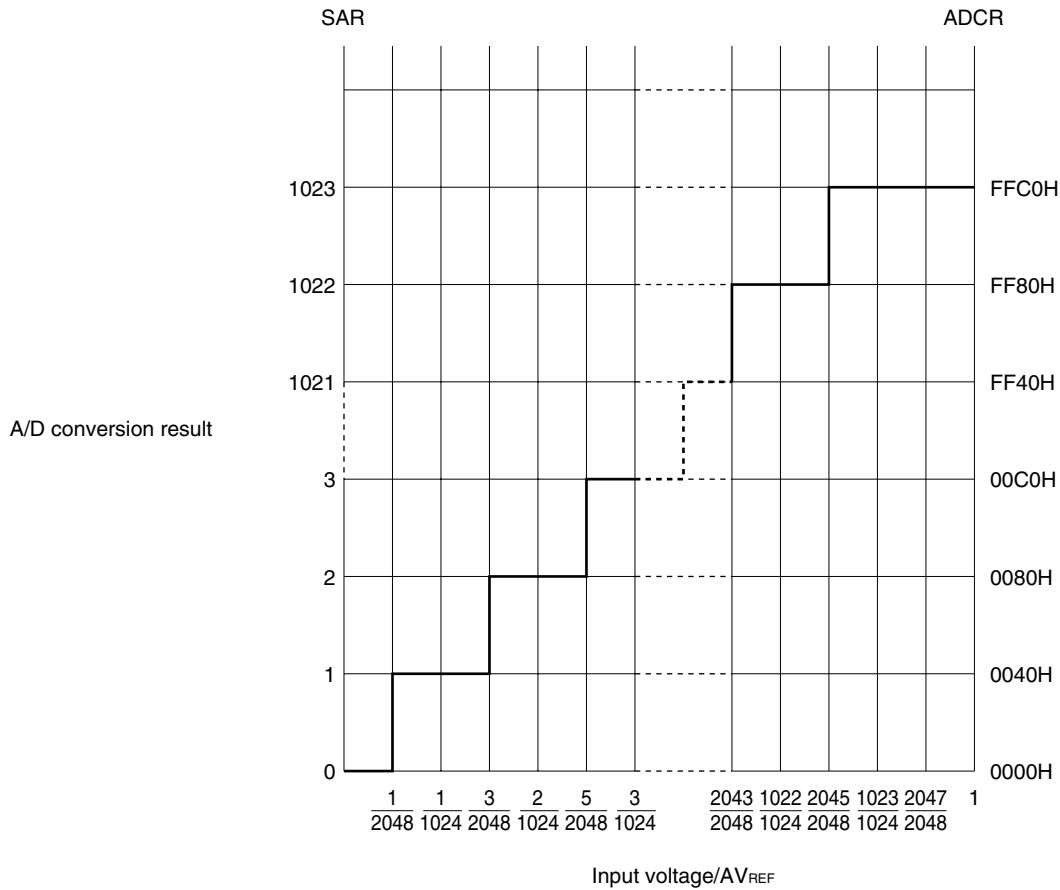
Figure 11-10. Relationship Between Analog Input Voltage and A/D Conversion Result
