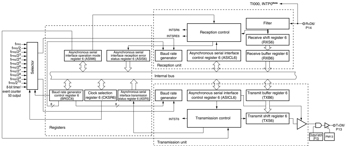
Figure 15-4. Block Diagram of Serial Interface UART6
