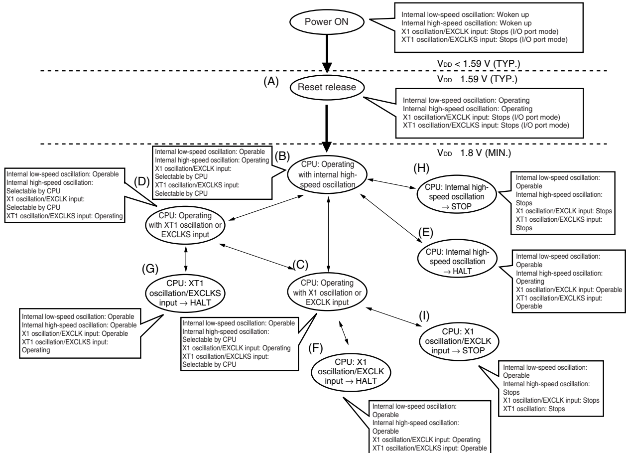
Figure 6-14. CPU Clock Status Transition Diagram (When 1.59 V POC Mode Is Set (Option Byte: POCMODE = 0))
