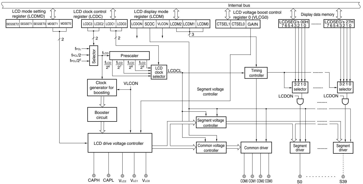
Figure 18-2. Block Diagram of LCD Controller/Driver
