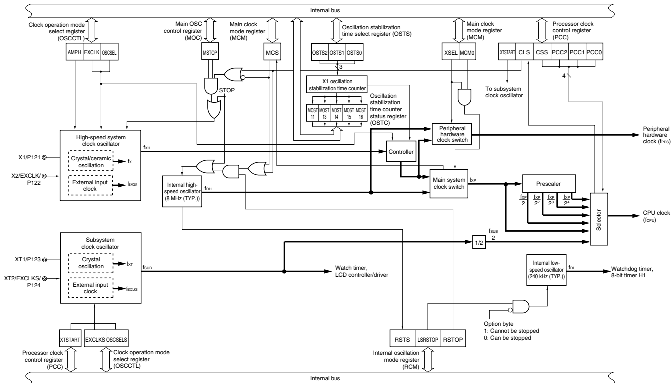
<R> Figure 6-1. Block Diagram of Clock Generator
