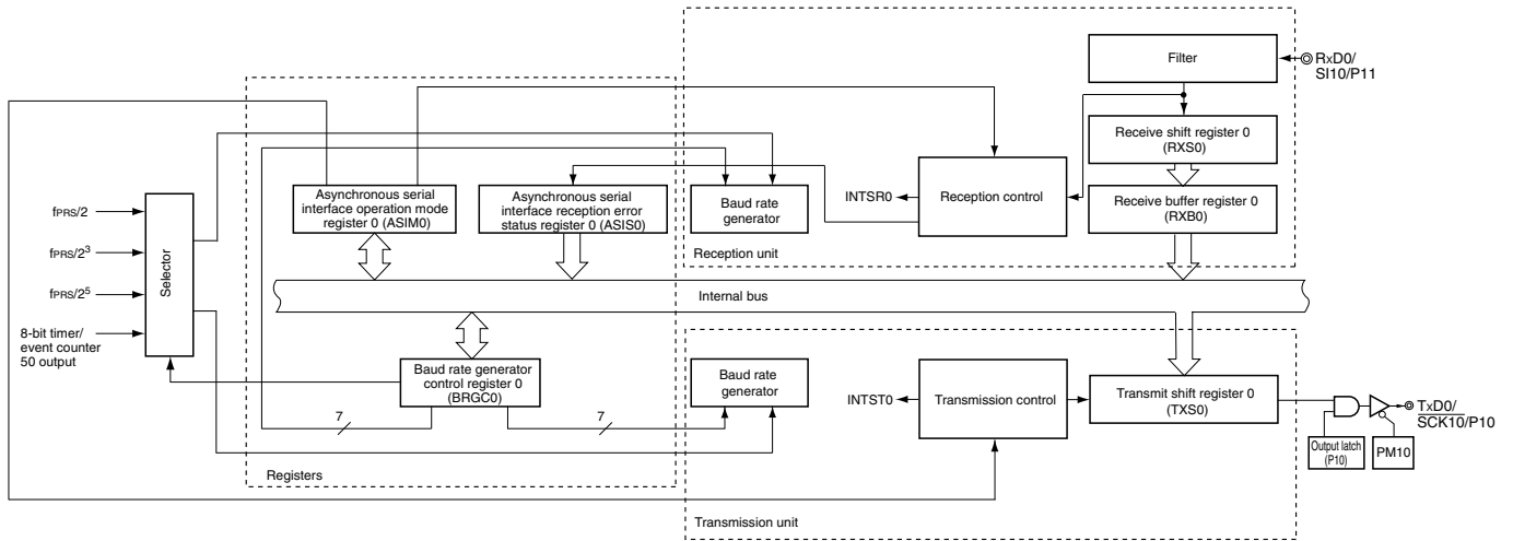
Figure 14-1. Block Diagram of Serial Interface UART0
