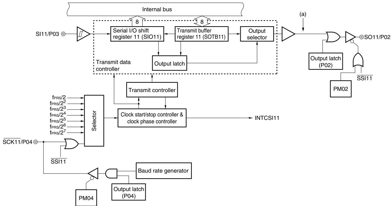
Figure 16-2. Block Diagram of Serial Interface CSI11 (Available only in the \mu PD78F0394, 78F0395, 78F0396, 78F0397, 78F0397D)
