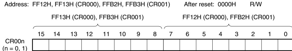
Figure 7-4. Format of 16-Bit Timer Capture/Compare Register 00n (CR00n)
