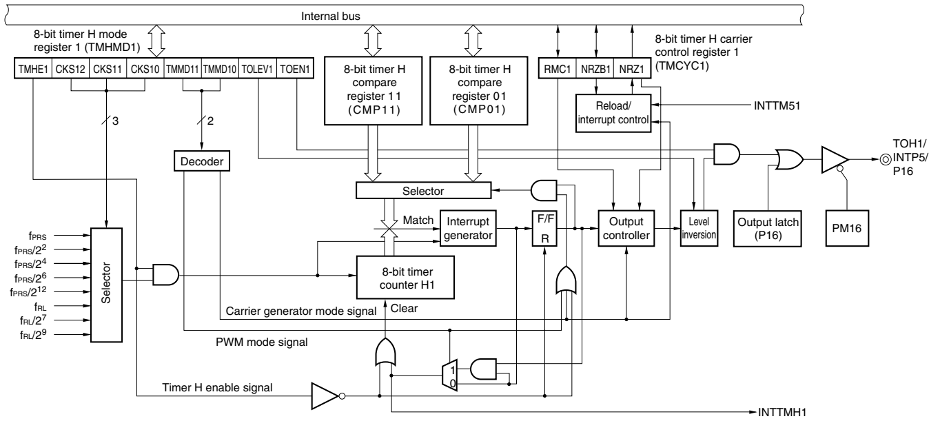
Figure 9-2. Block Diagram of 8-Bit Timer H1
