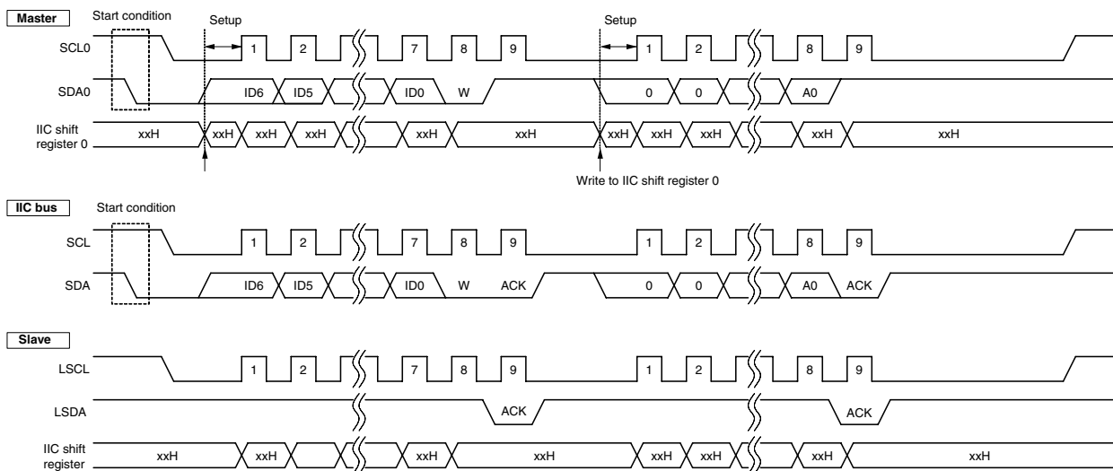
Figure 17-36. Timing Chart of Read Operation
