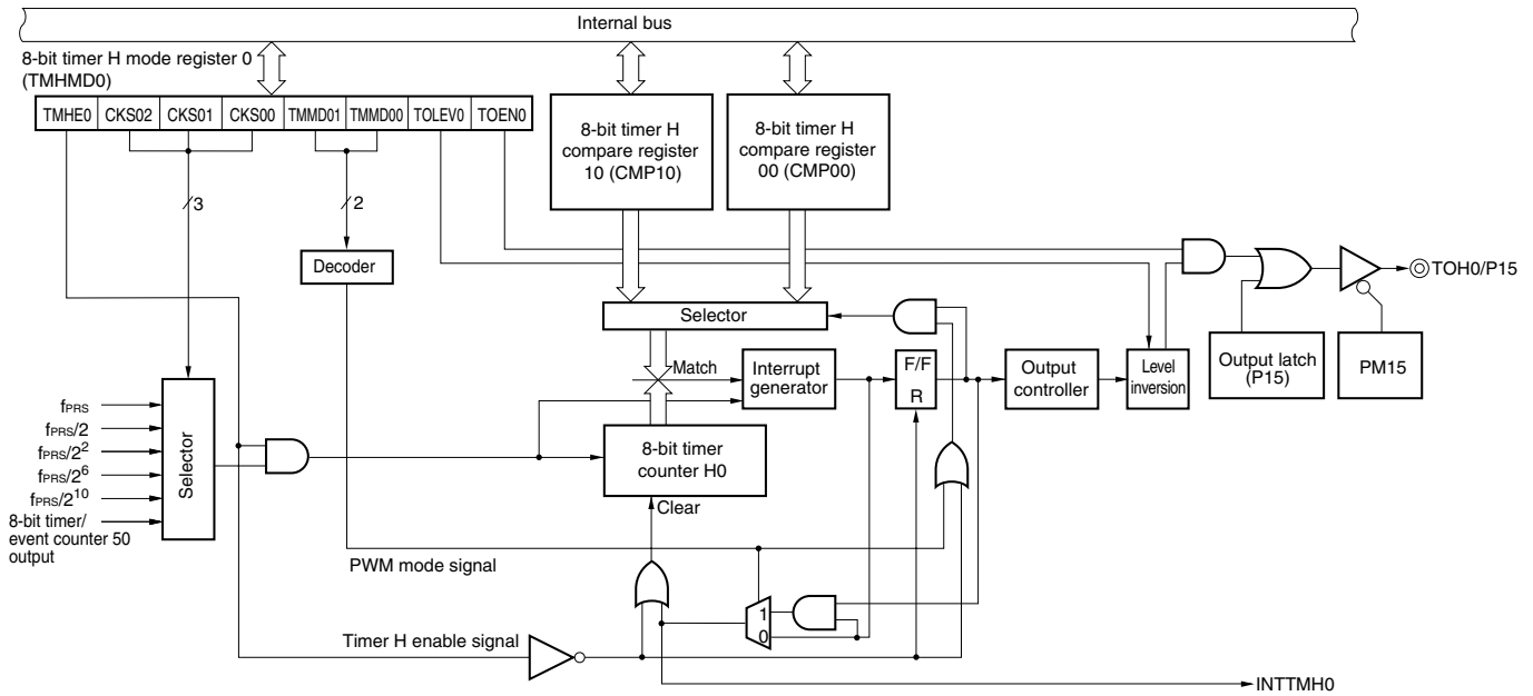
Figure 9-1. Block Diagram of 8-Bit Timer H0
