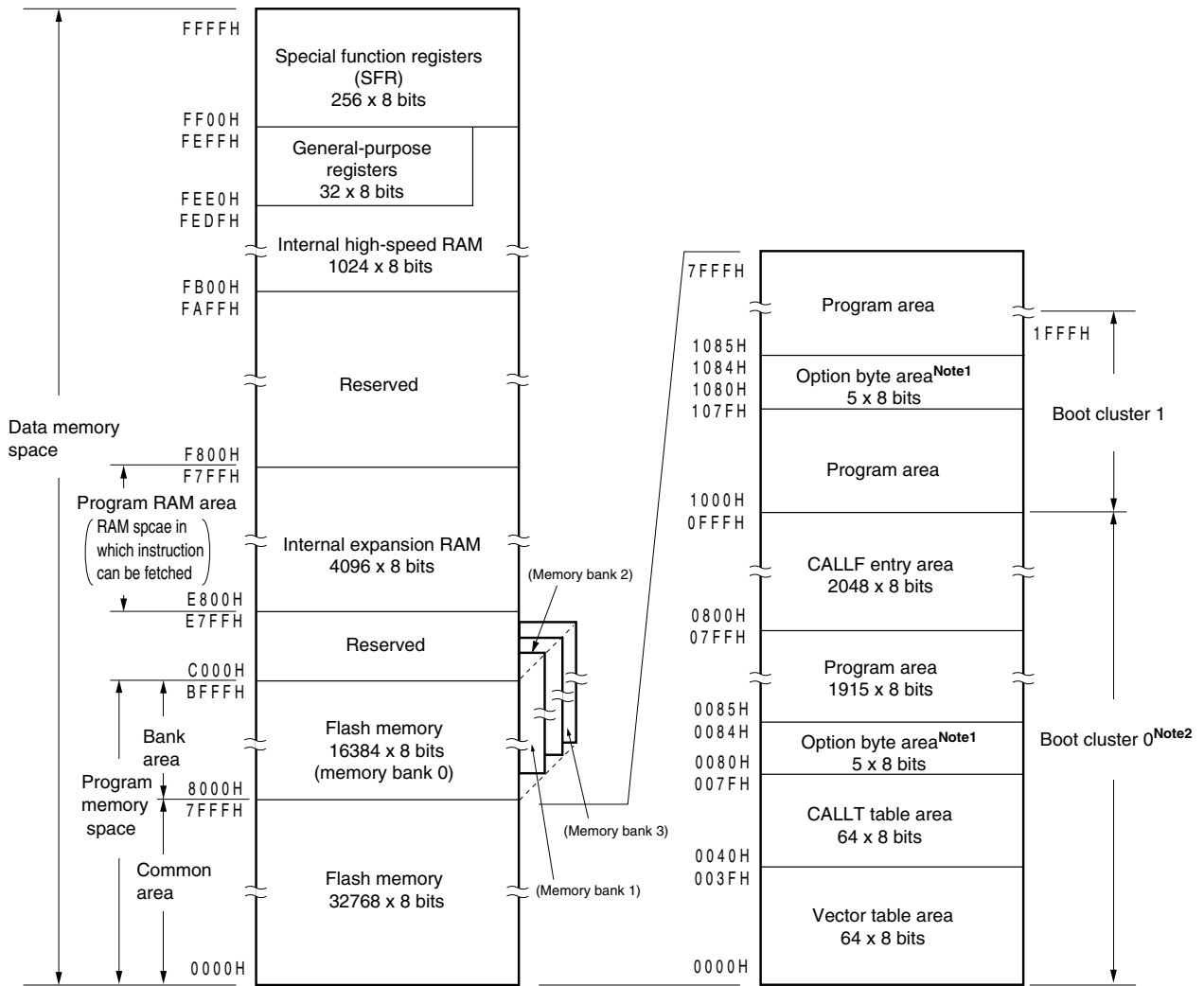
Figure 3-4. Memory Map ( \mu PD78F0396)
