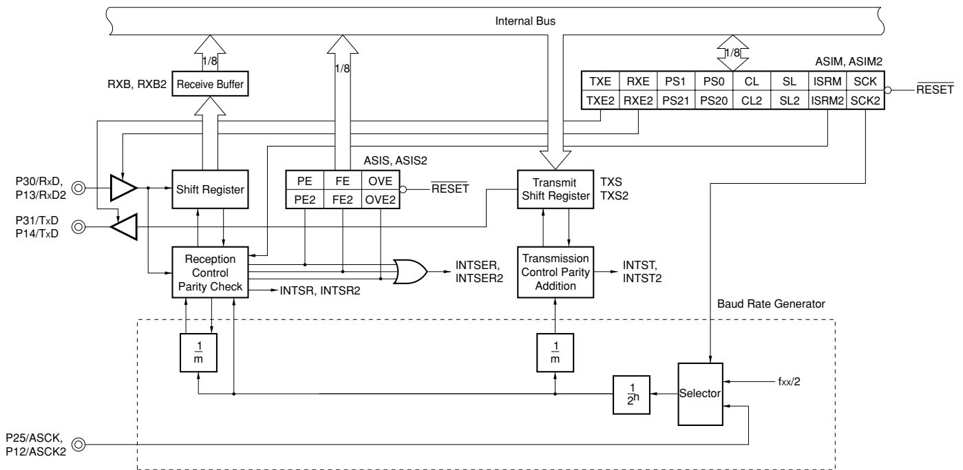
Figure 17-2 Asynchronous Serial Interface Block Diagram
