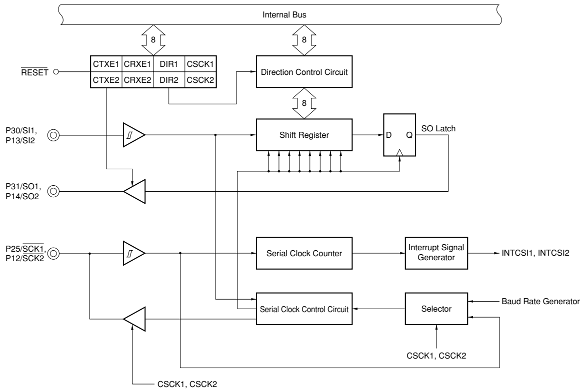
Figure 17-10 3-Wire Serial I/O Mode Block Diagram
