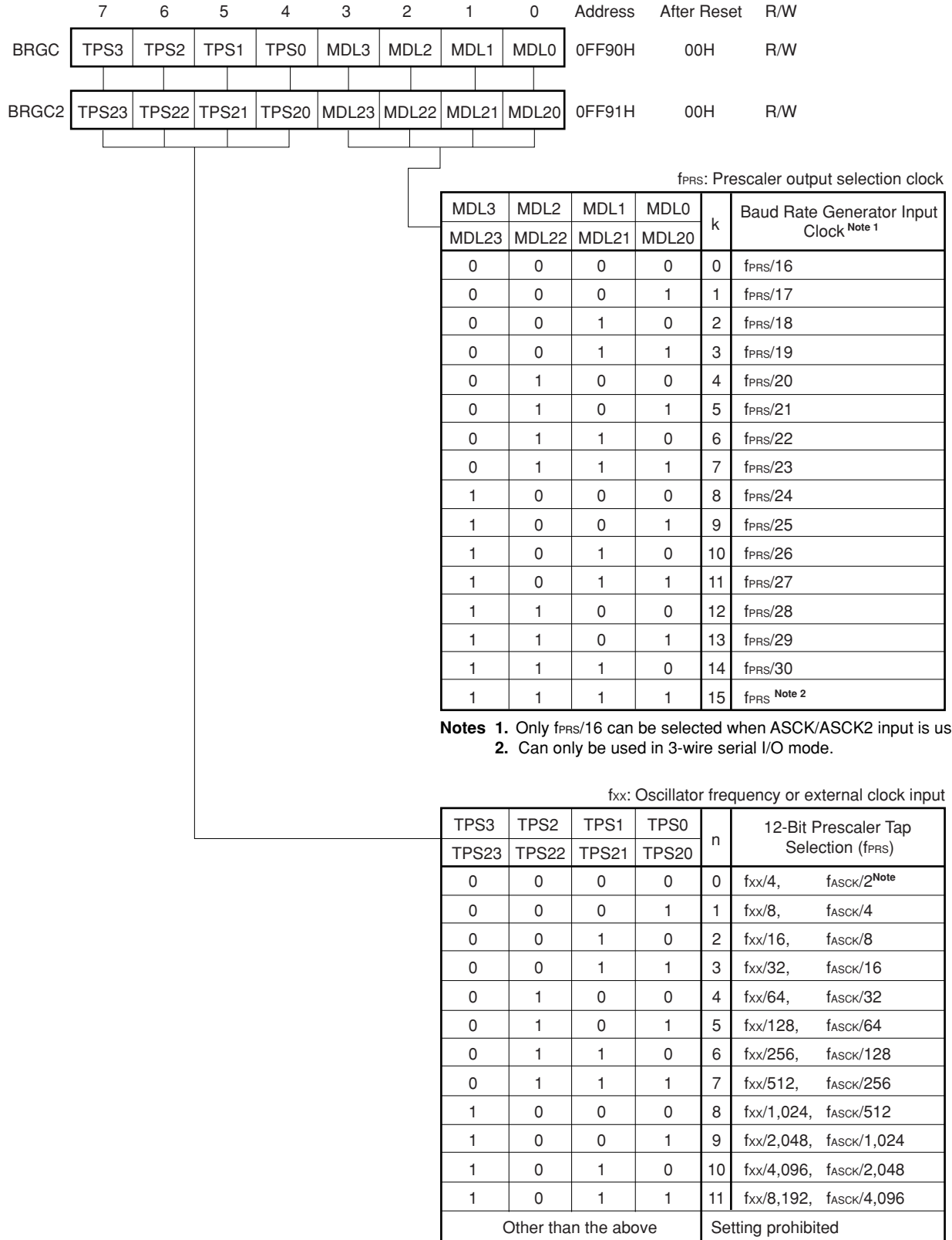
Figure 17-15 Baud Rate Generator Control Register (BRGC) Format and Baud Rate Generator Control Register 2 (BRGC2) Format
