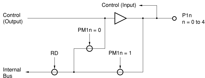
Figure 5-18 Control Specification
