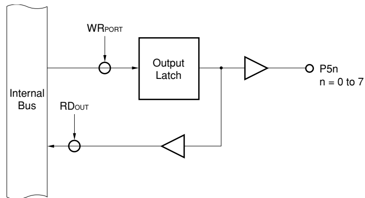
Figure 5-47 Port Specified as Output Port
