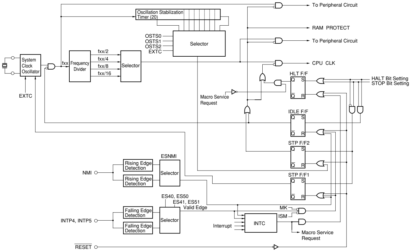
Figure 24-2 Standby Function Block Diagram
