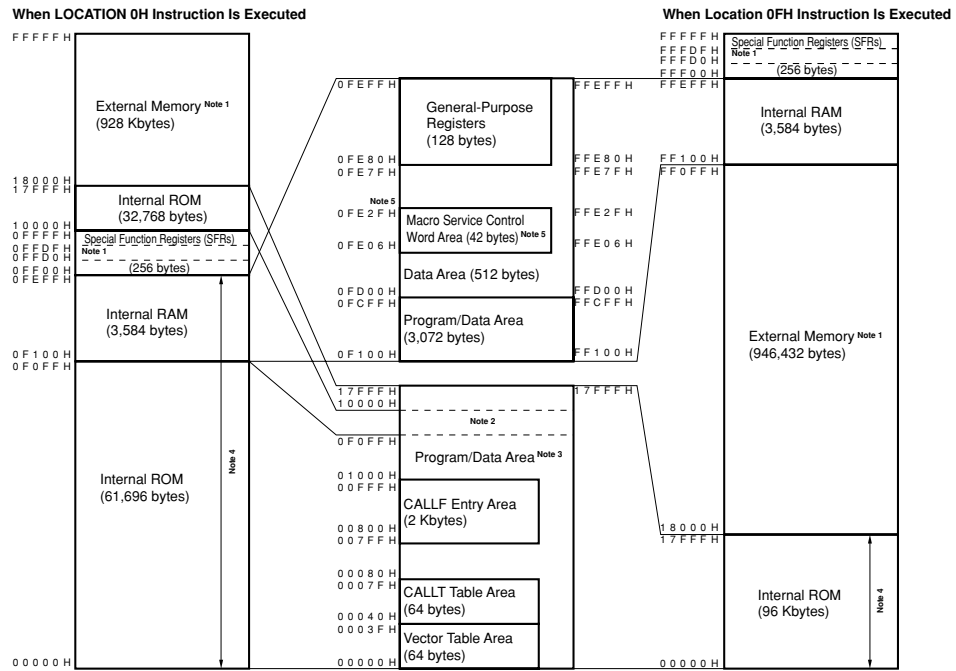
Figure 3-4 \mu PD784037 Memory Map
