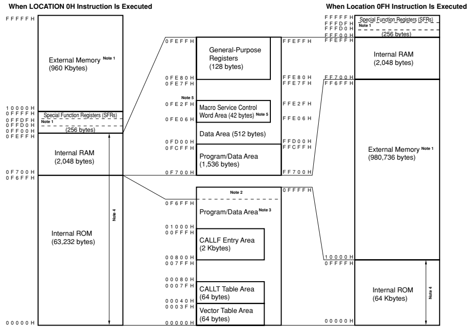
Figure 3-3 \mu PD784036 Memory Map
