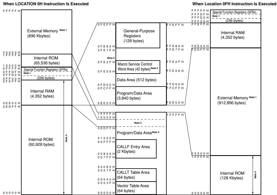
Figure 3-5 \mu PD784038 Memory Map
