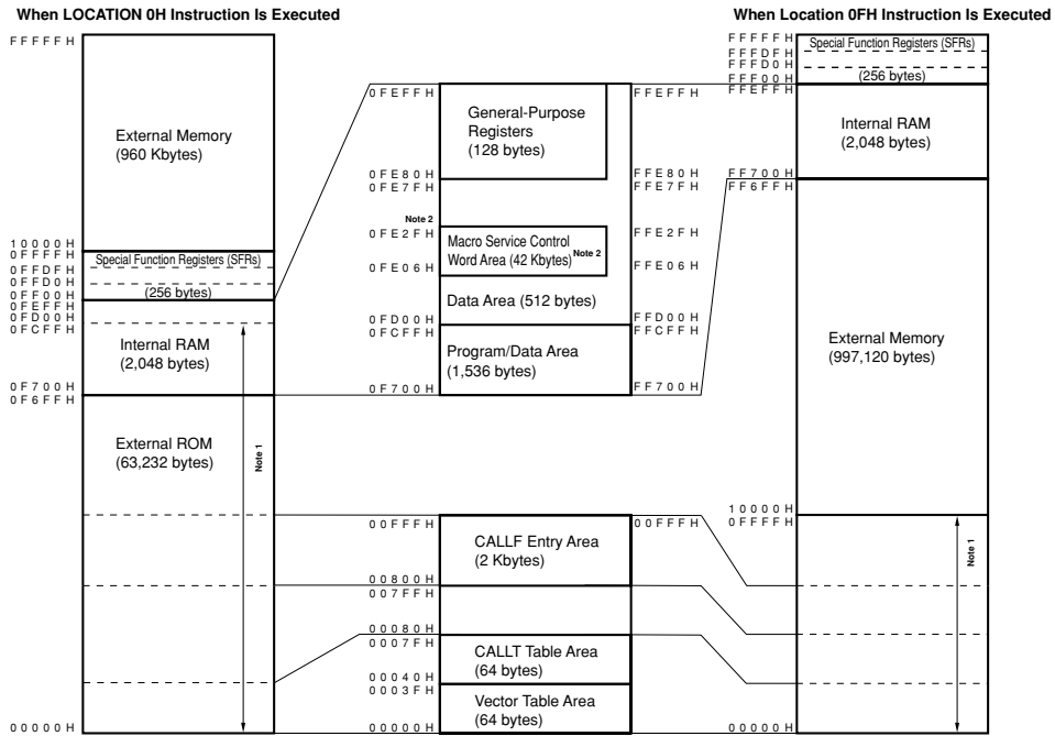
Figure 3-1 \mu PD784031 Memory Map
