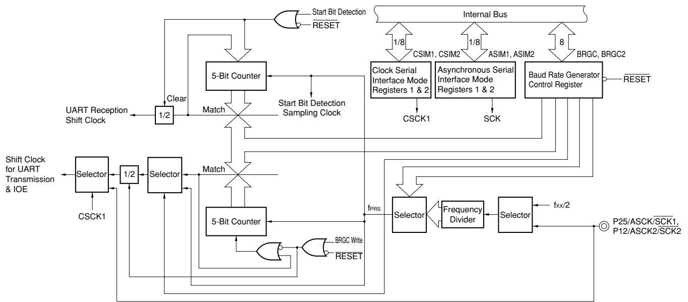
Figure 17-14 Baud Rate Generator Block Diagram
