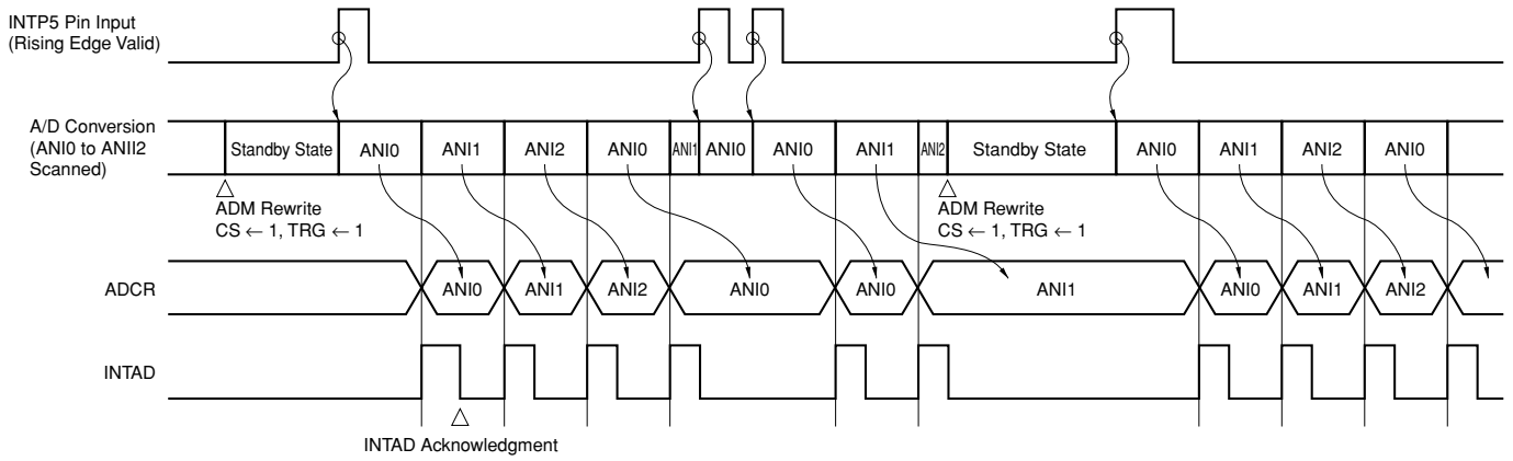
Figure 14-12 Hardware Start Scan Mode A/D Conversion Operation
