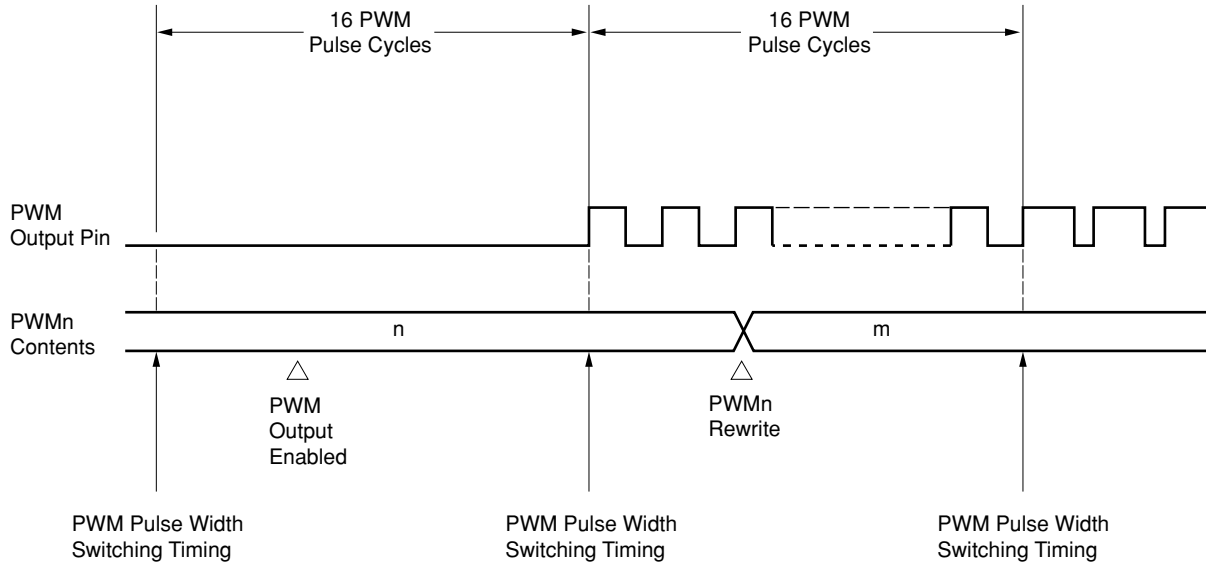
Figure 13-6 PWM Output Timing Example 1 (PWM Pulse Width Rewrite Cycle = 2^{12}/f_{\text{PWM}} )
