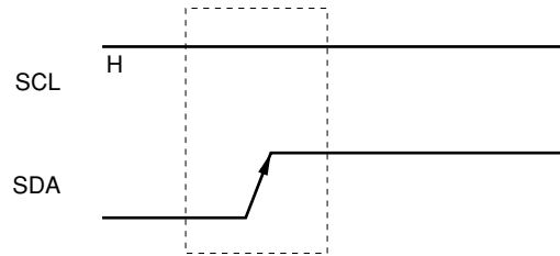
Figure 19-13 Stop Condition
