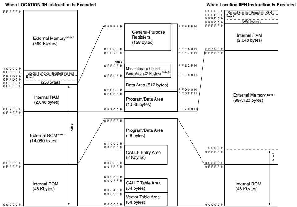
Figure 3-2 \mu PD784035 Memory Map
