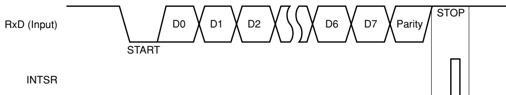
Figure 17-7 Asynchronous Serial Interface Reception Completion Interrupt Timing
