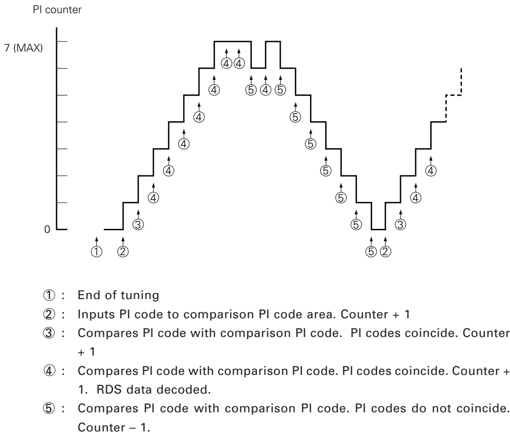
Fig. 4-1 PI Counter Operation
