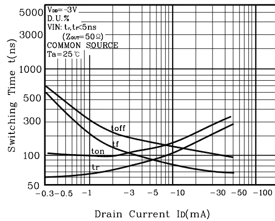
Fig8 t - Id
