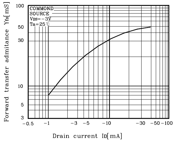
Fig5 | Yfs | - Id
