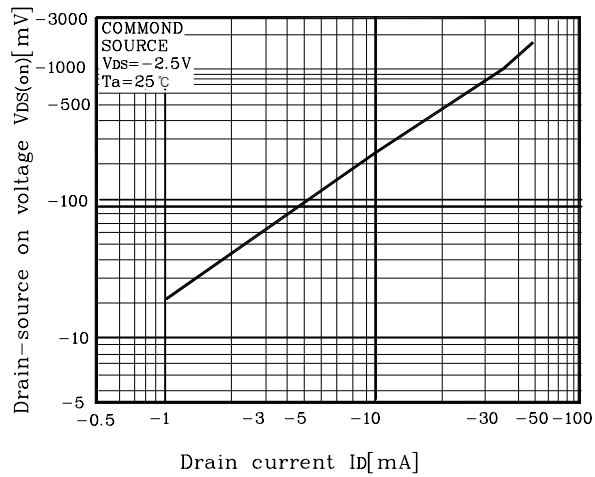
Fig7 VDS(on) - Id
