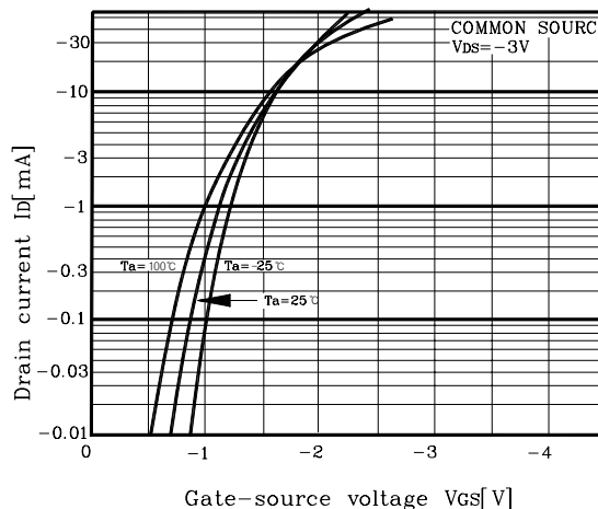
Fig4 I D - V GS
