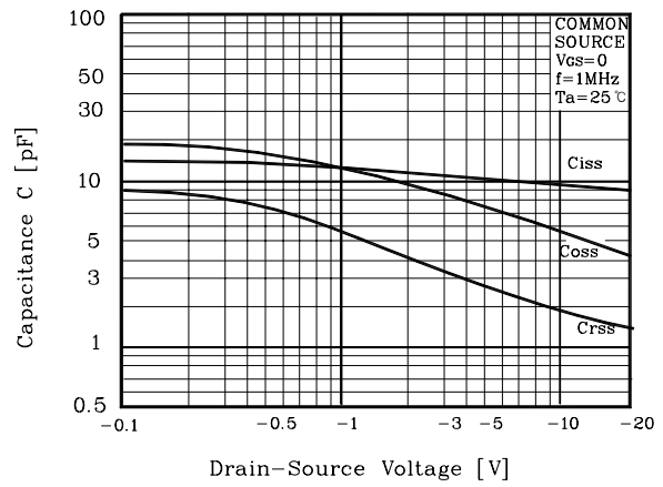
Fig6 C - Vds
