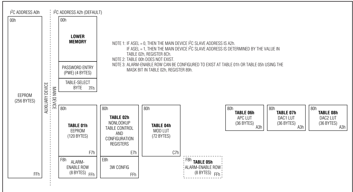
Figure 21. Memory Map
