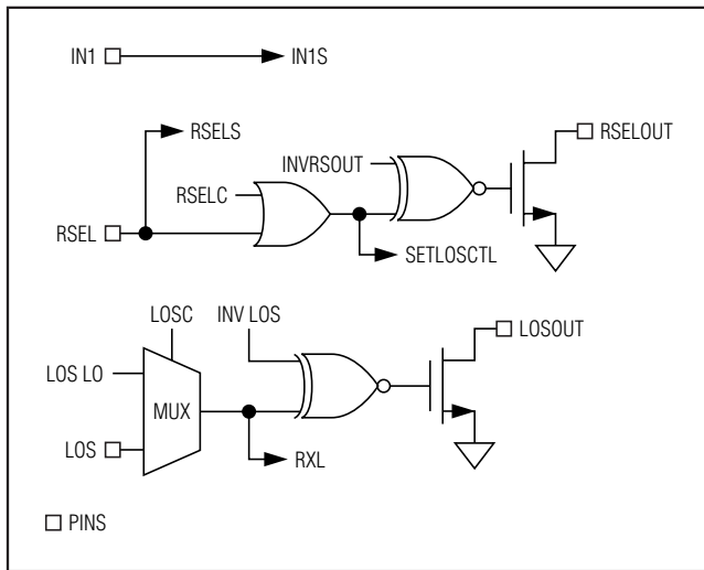
Figure 15. Logic Diagram 2
