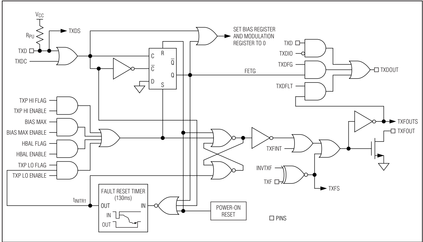
Figure 14. Logic Diagram 1
