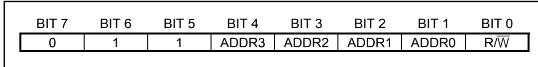
Figure 25. DS2786 I 2 C Address Byte Format
