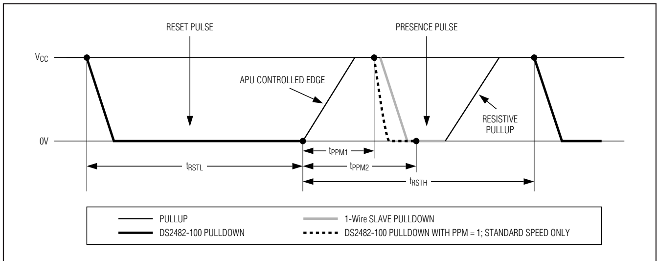
Figure 3. Presence-Pulse Masking
