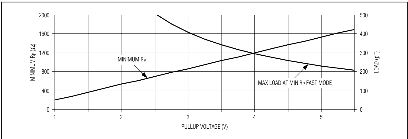
Figure 12. I²C Fast Speed Pullup Resistor Selection Chart
