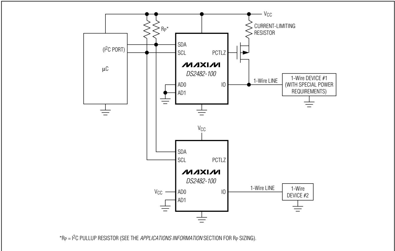
Figure 11. Application Schematic
