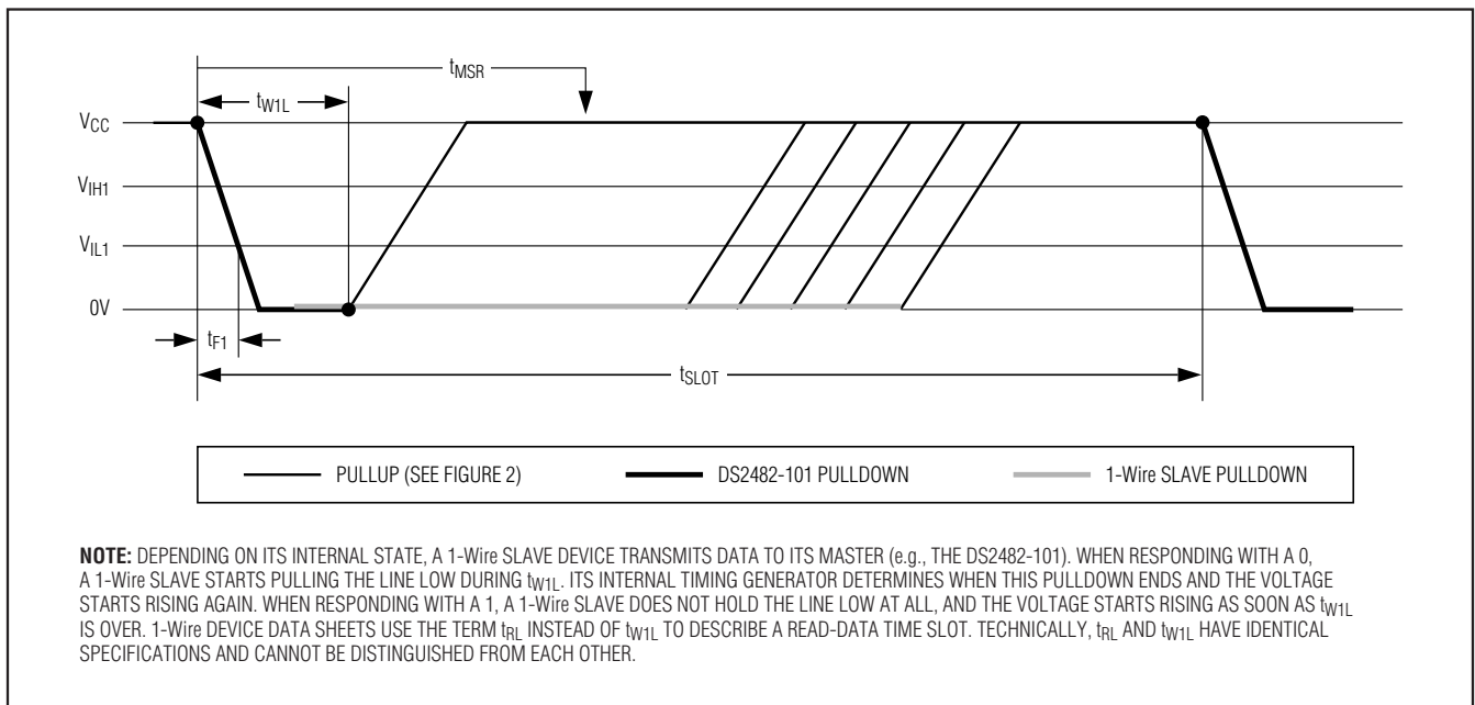
Figure 7. Write-One and Read-Data Time Slot
