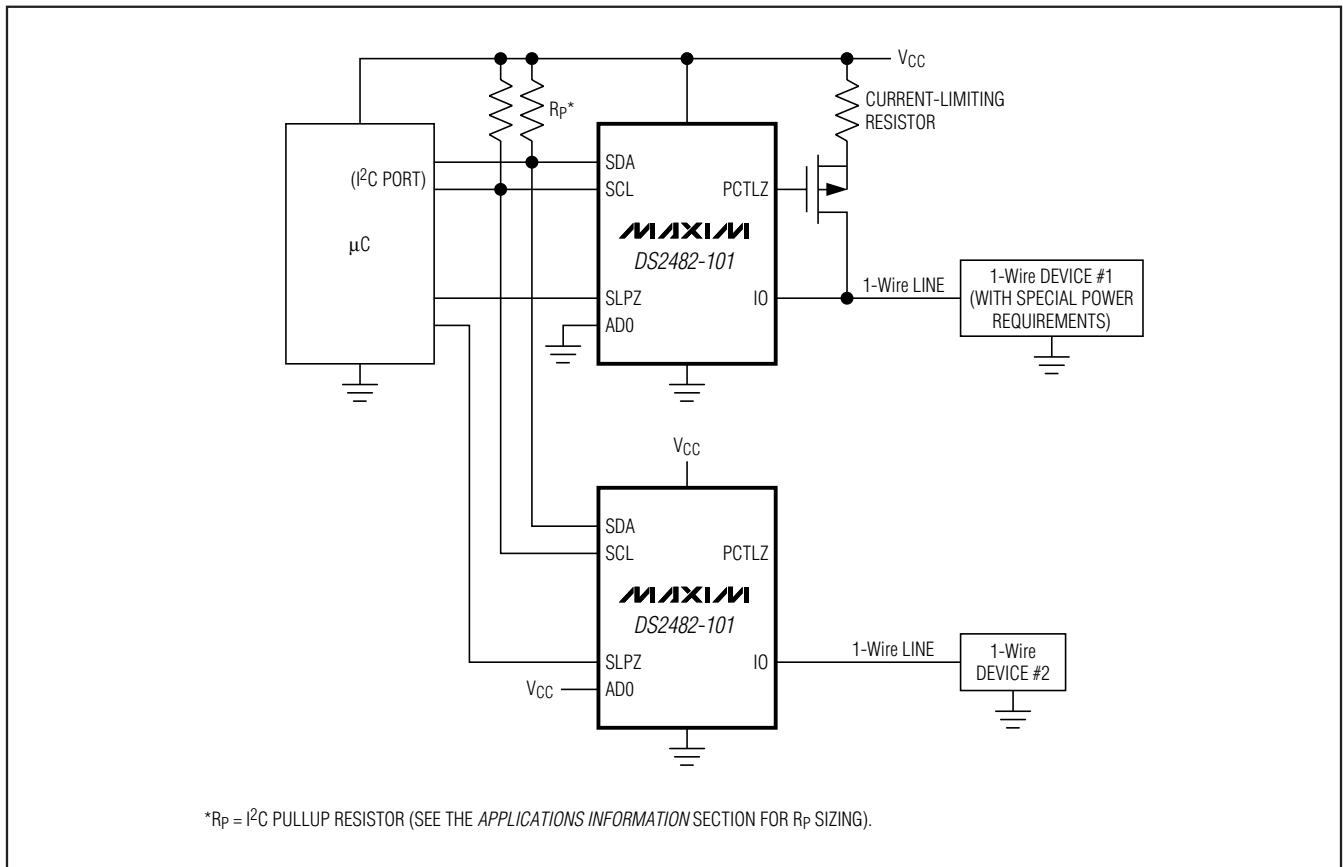
Figure 11. Application Schematic
