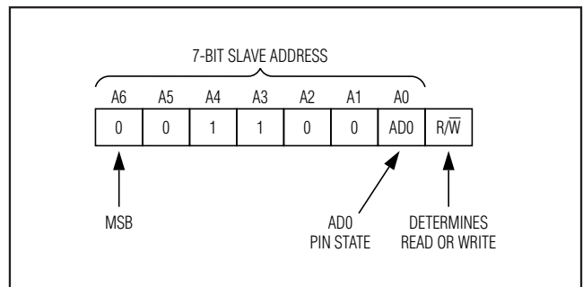
Figure 9. DS2482-101 Slave Address
