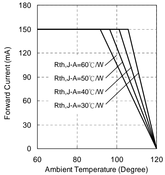
Fig 4. Forward Current Derating Curve
