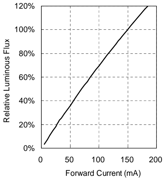
Fig 5. Relative Luminous Flux
