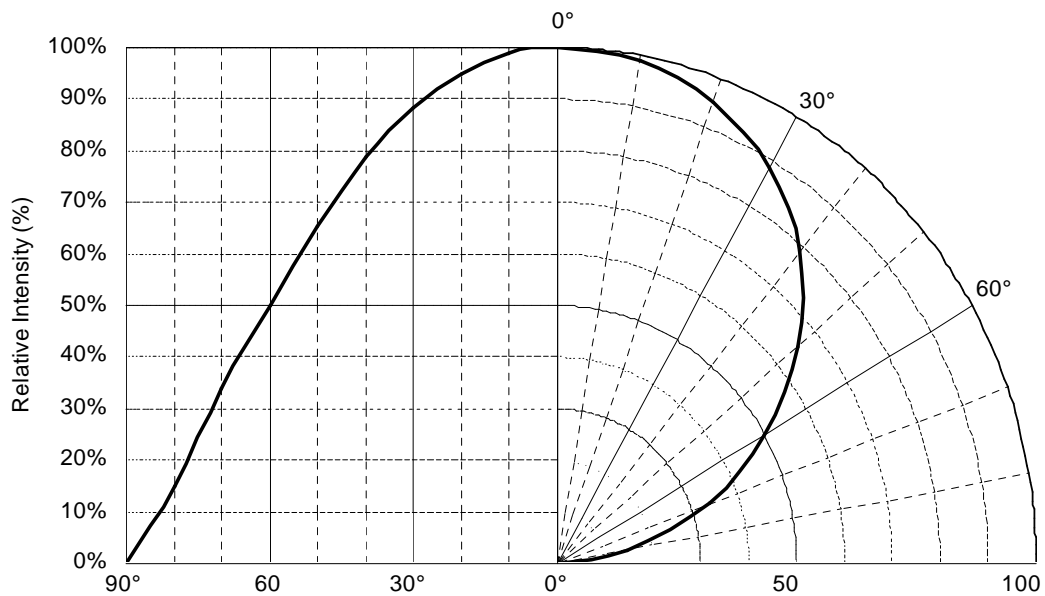
Fig 2. Radiation Characteristics
