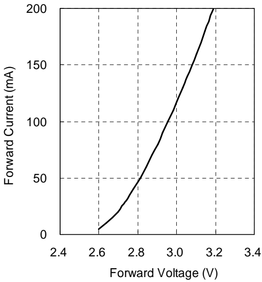
Fig 3. Forward Current
