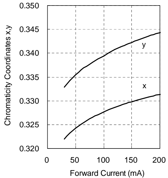
Fig 6. Chromaticity Coordinate Shift
