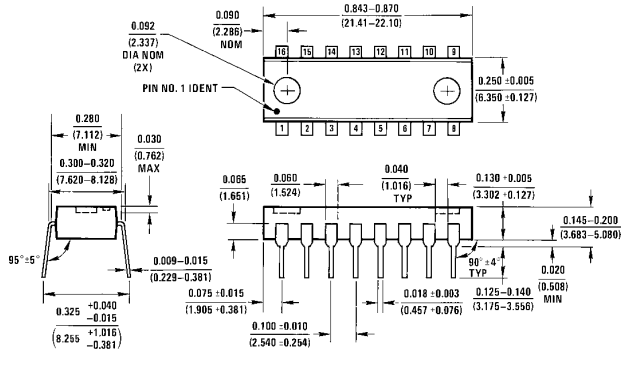
Molded Dual-In-Line Package (N) Order Number DS8837N NS Package Number N16A
