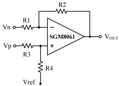
Figure 3. Differential Amplifier
