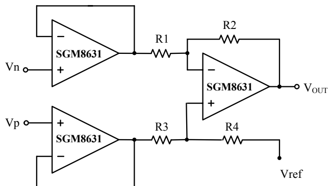
Figure 5. Instrumentation Amplifier
