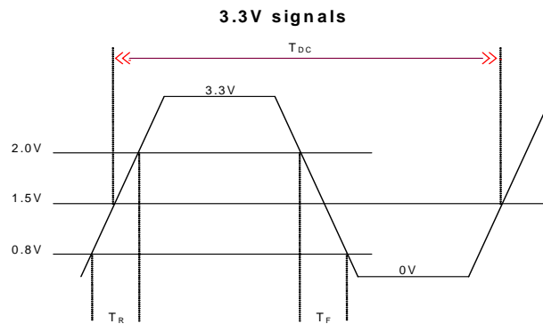
Figure 16. Single-ended Output Signals (for AC Parameters Measurement)
