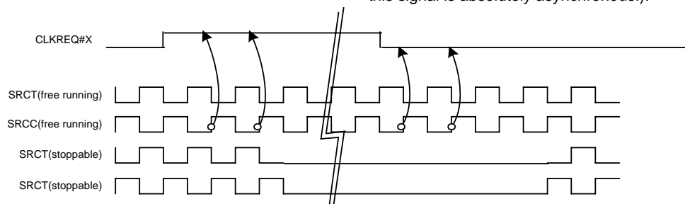
Figure 3. CLK_REQ# Deassertion/Assertion Waveform
