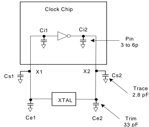
Figure 2. Crystal Loading Example
