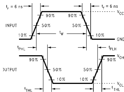
FIGURE 3. AC Waveforms
