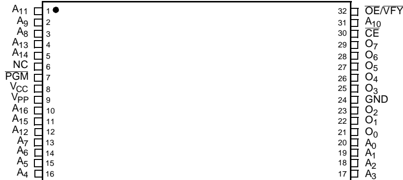
TSOP Top View
