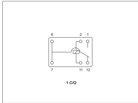
Connection diagram (pin side view)
